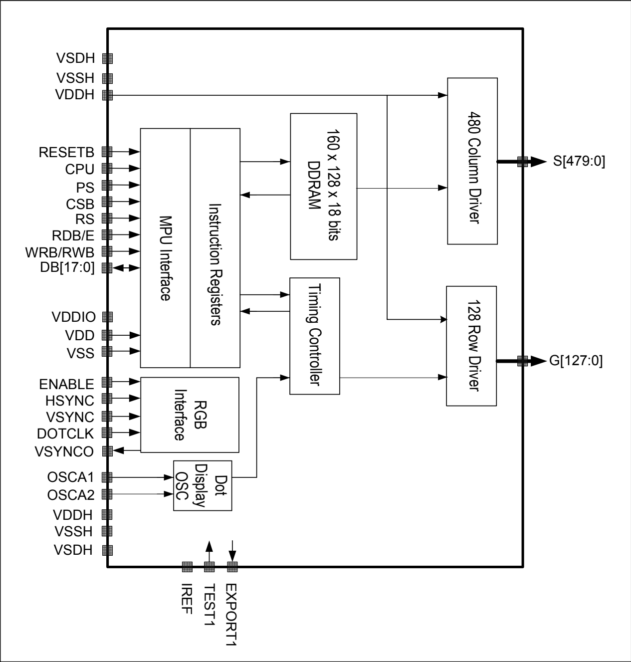
Block Diagram
