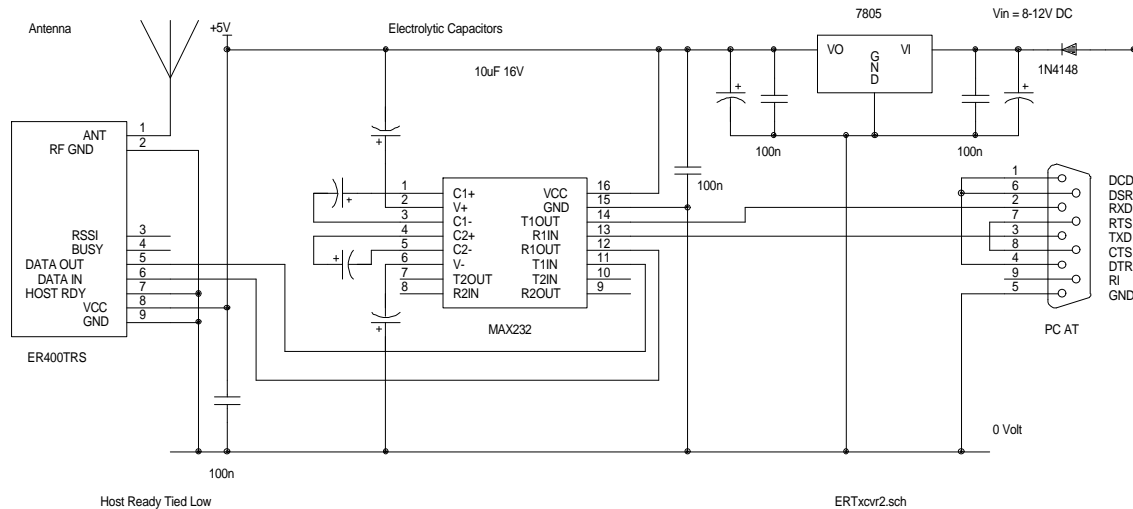
Figure 3 Application Circuit
