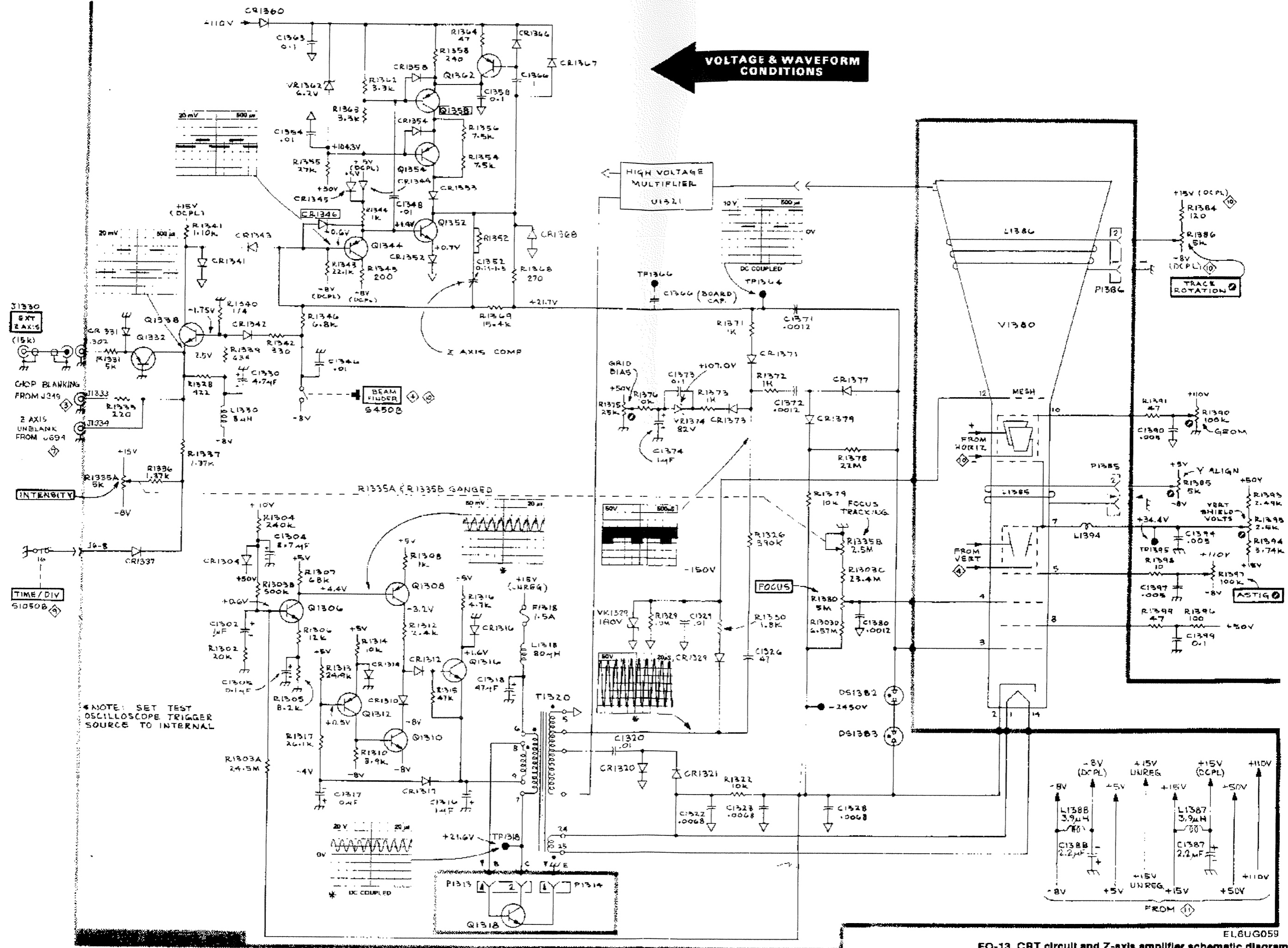
CRT CIRCUIT & Z-AXIS AMPLIFIER
