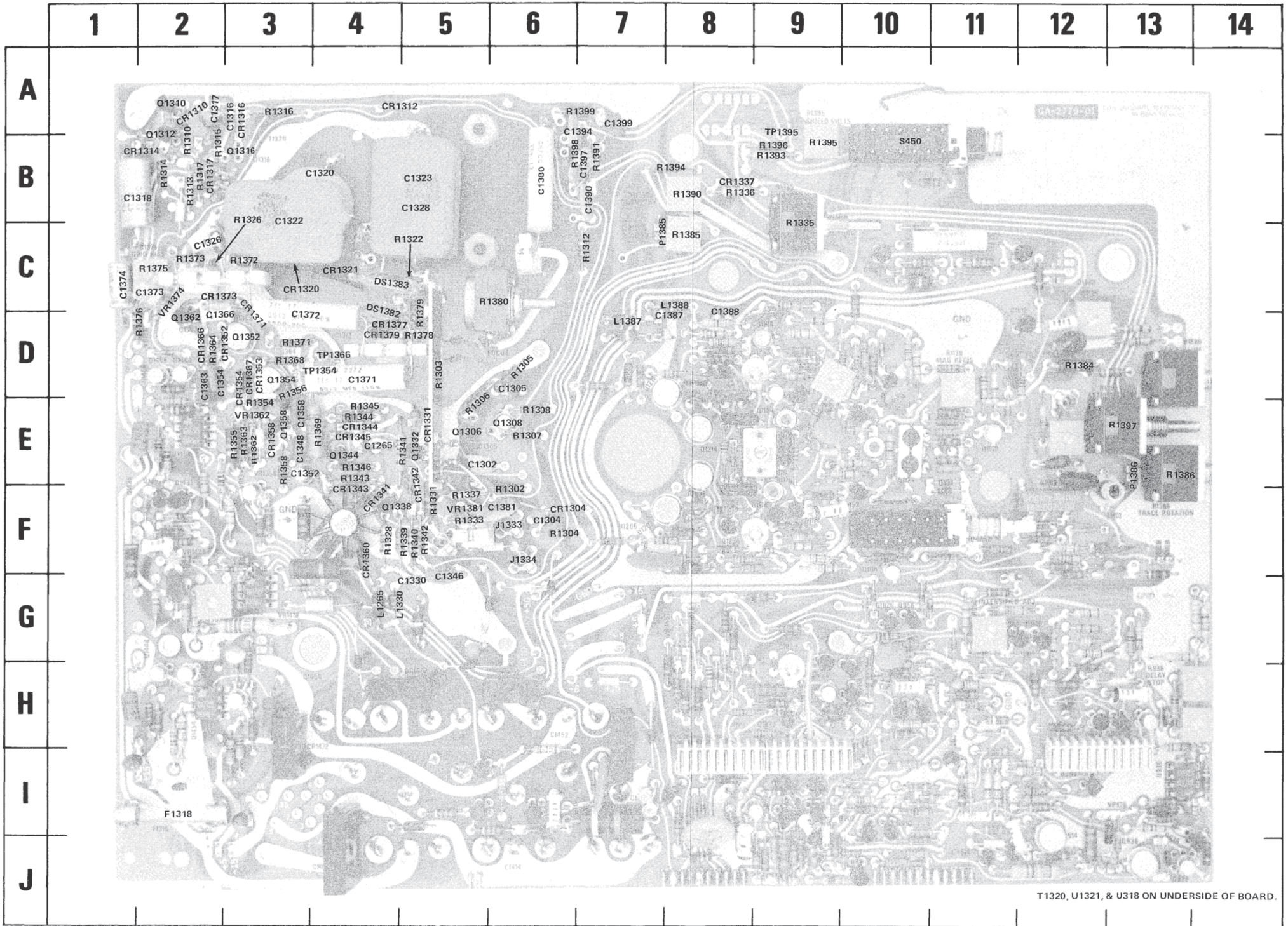
Fig. 7-19. P/O A9 Interface circuit board.
