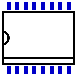
SO16W_SOT162-1
