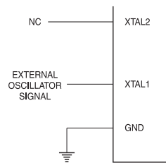
Figure 16-4. External Clock Drive Configuration
