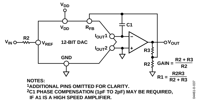
Figure 37. Increasing the Gain of the Current Output DAC
