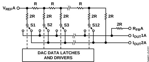
Figure 32. Simplified Ladder
