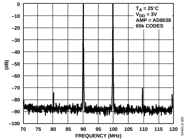
Figure 29. Narrow-Band IMD, f_{OUT} = 90\text{ kHz}, 100\text{ kHz} , Clock = 10 MHz
