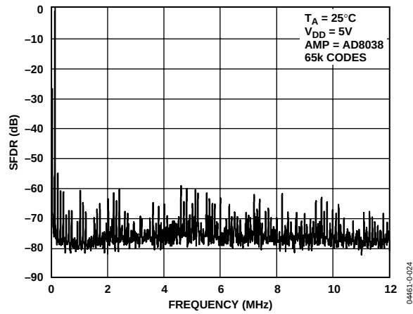
Figure 24. Wideband SFDR, f_{OUT} = 100\text{ kHz} , Clock = 25 MHz
