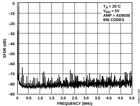
Figure 26. Wideband SFDR, f_{OUT} = 50\text{ kHz} , Clock = 10 MHz
