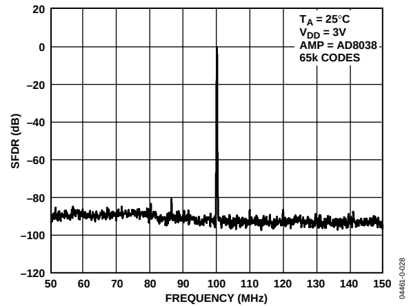
Figure 28. Narrow-Band SFDR, f_{OUT} = 100\text{ kHz} , MCLK = 25 MHz
