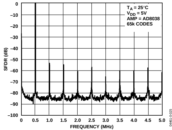
Figure 25. Wideband SFDR, f_{OUT} = 500\text{ kHz} , Clock = 10 MHz
