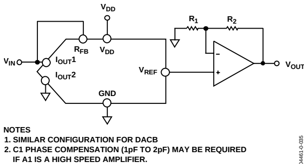
Figure 35. Single-Supply Voltage Switching Mode
