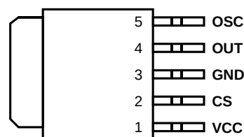
TO-252-5L (Top View)
