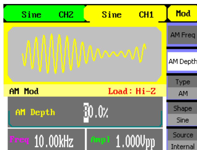
Figure 3-9 AM Waveform
