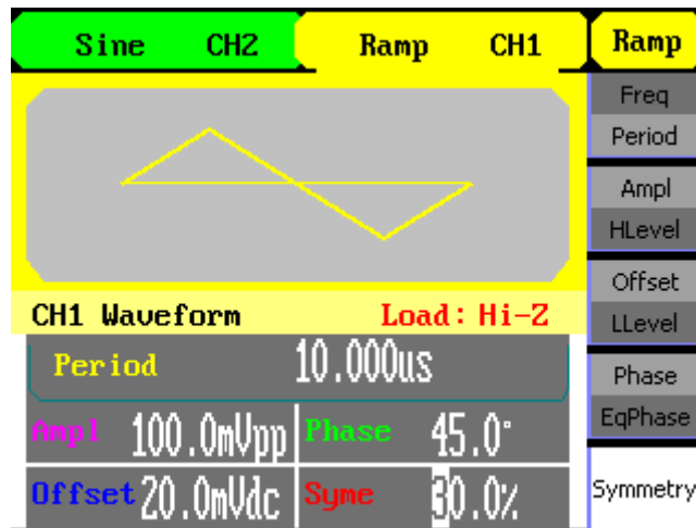
Figure 3-3 Ramp Waveform
