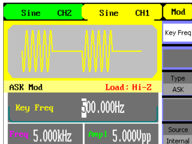
Figure 3-13 ASK Waveform
