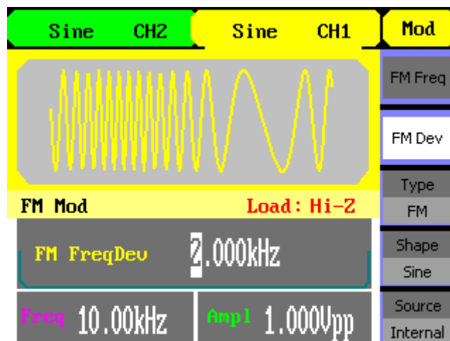
Figure 3-10 FM Waveform
