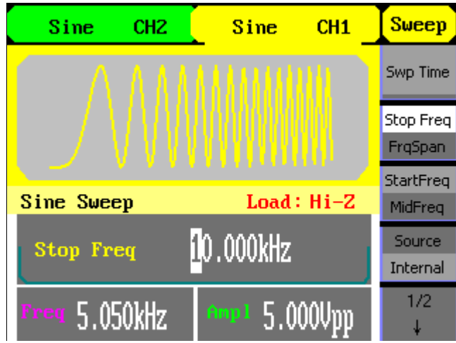
Figure 3-7 Sweep Waveform
