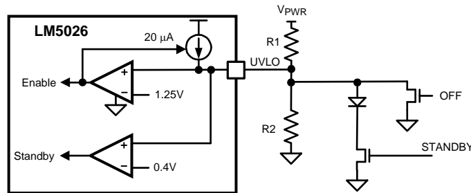
Figure 17. Remote Standby and Disable Control
