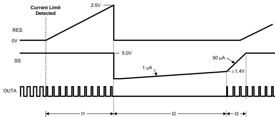
Figure 10. Hiccup Over-Load Restart Timing
