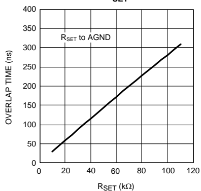
Deadtime vs R_{SET}
