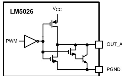
Figure 6. Compound Gate Driver
