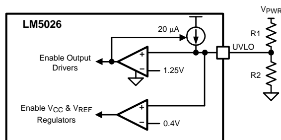
Figure 16. Basic UVLO Configuration
