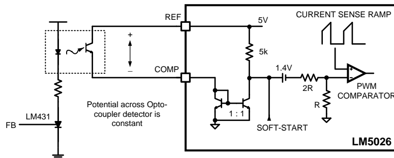
Figure 7. Opto-Coupler to LM5026 COMP Interface
