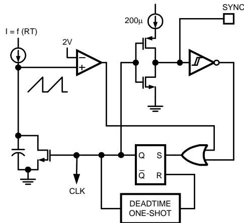
Figure 13. Oscillator Sync I/O Block Diagram
