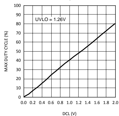
Max Duty Cycle vs DCL
