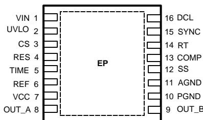
Figure 3. 16-Lead Thermally Enhanced
