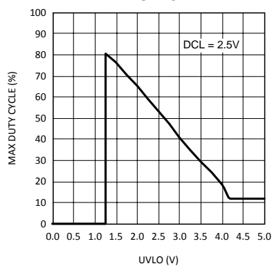
Max Duty Cycle vs UVLO
