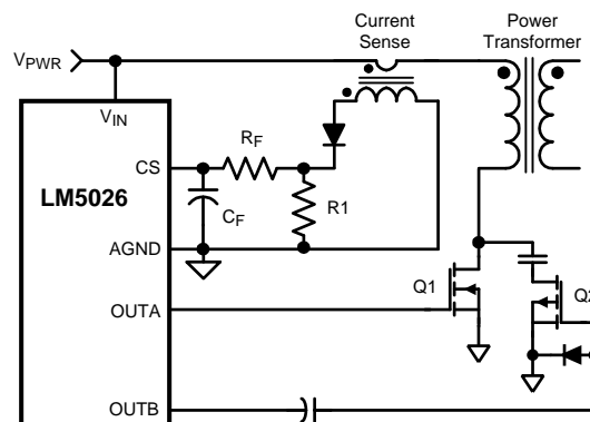
Figure 18. Current Sense Using a Current Sense Transformer
