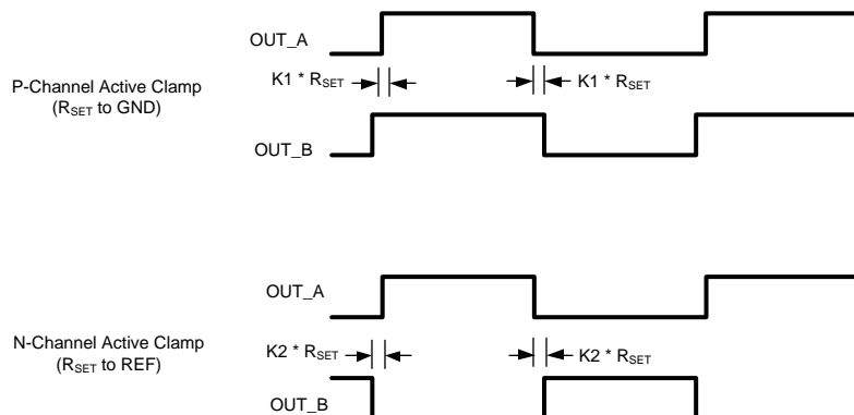
Figure 5. PWM Output Phasing / Timing
