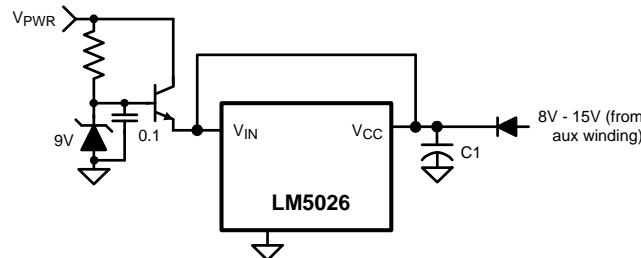
Figure 15. Start-Up Regulator for V_{PWR} > 100V
