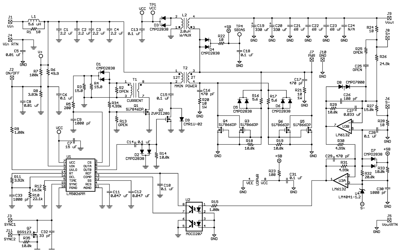
Figure 21. Application Circuit: Input 36-78V, Output 3.3V, 30A
