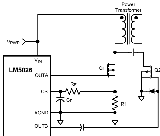
Figure 19. Current Sense Using a Source Sense Resistor (R1)
