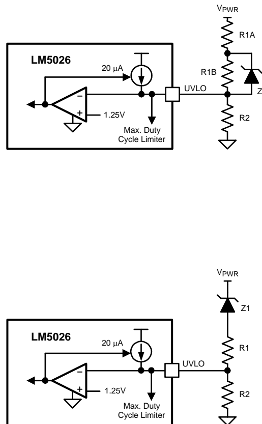
Figure 20. Altering the Slope of Duty Cycle vs. V_{PWR}
