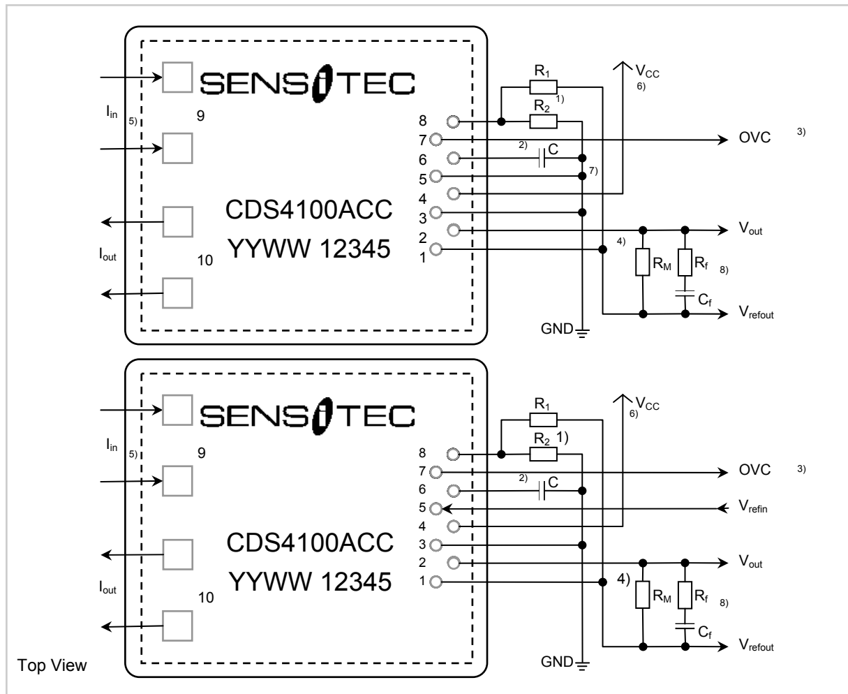
Fig. 7: Top : Example of how to use the internal reference voltage (pin 5, V_{refin} is routed on ground).
