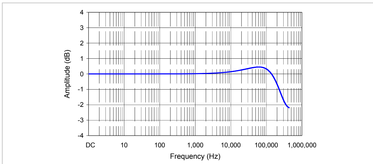
Fig. 11: Typical frequency response without using a RC-Filter.
