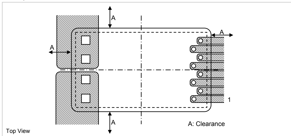
Fig. 9: Recommended PCB layout for the CDS4100 sensor (schematic).
