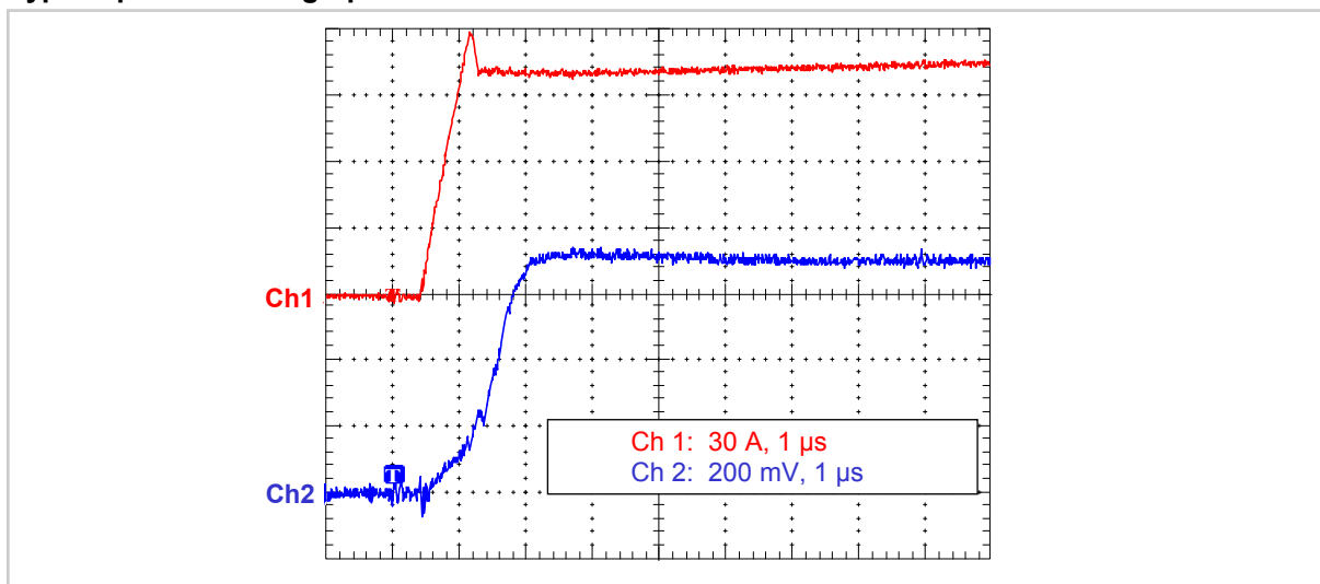
Fig. 10: Typical output characteristic due to a current jump from 0 to I_{PN} . Input di/dt \approx 150\text{ A}/\mu\text{s} . An RC-Filter with the parameters R_F = 1.5\text{ k}\Omega and C_F = 22\text{ nF} ( R_M = 300\text{ }\Omega ) is used.
