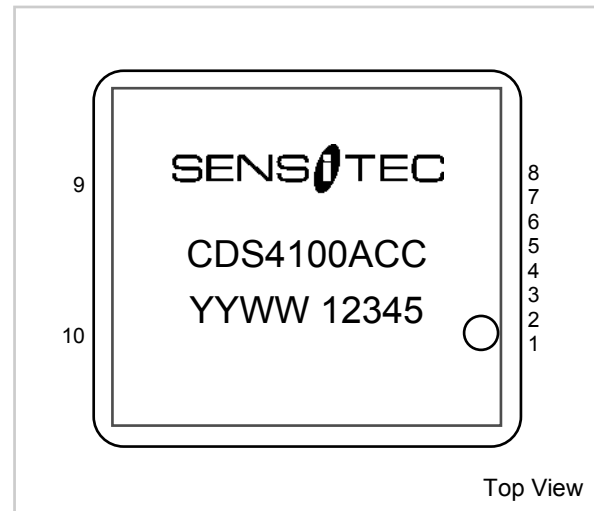
Fig. 5: Pinning of CDS4100ACC.
