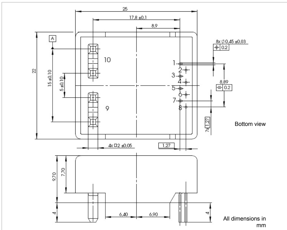
Fig. 6: Package outline of THT-housing. Tolerance \pm 0.2 mm unless otherwise specified.
