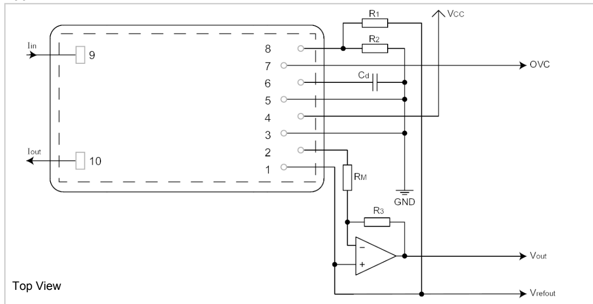
Fig. 8: Example of how to use an operational amplifier to adjust the output signal to an A/D converter. With R_M = 300 \, \Omega and R_3 = 410 \, \Omega , the output signal is amplified to a full scale output of 4.92 V.
