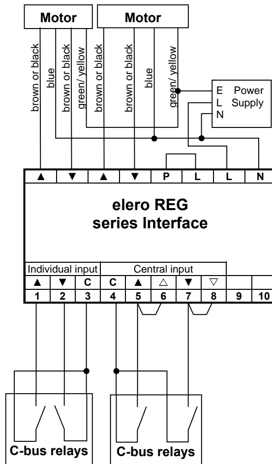
Picture shows 2-way REG. Other REG controllers are similar
