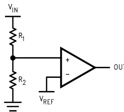
Figure 18. Threshold Detector
