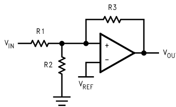
Figure 16. Additional Hysteresis
