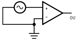
Figure 17. Zero-Crossing Detector
