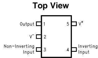
Figure 1. SC70 and SOT-23 Packages See Package Numbers DCK0005A and DBV0005A
