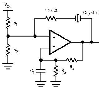
Figure 19. Crystal Oscillator
