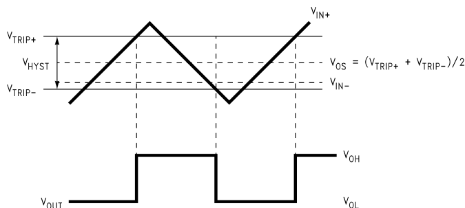
Figure 15. Input and Output Waveforms, Non-Inverting Input Varied
