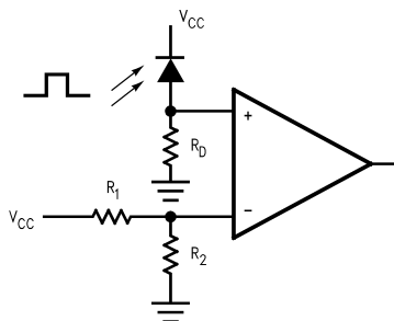
Figure 20. IR Receiver
