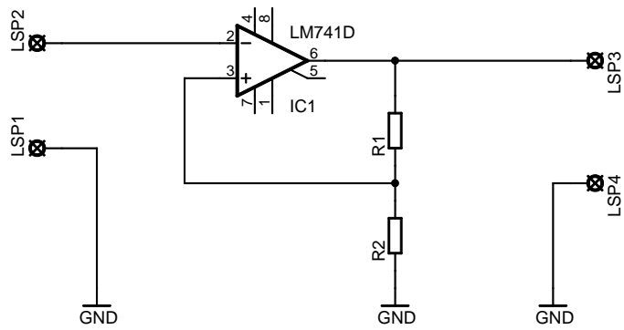
Invertierender Schmitt-Trigger
