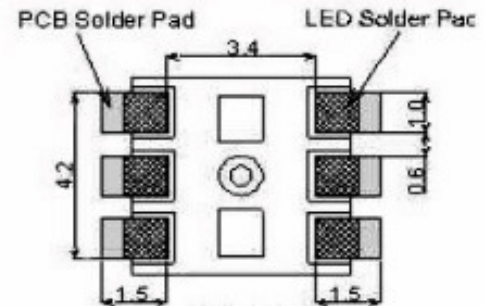
Solder Pad
