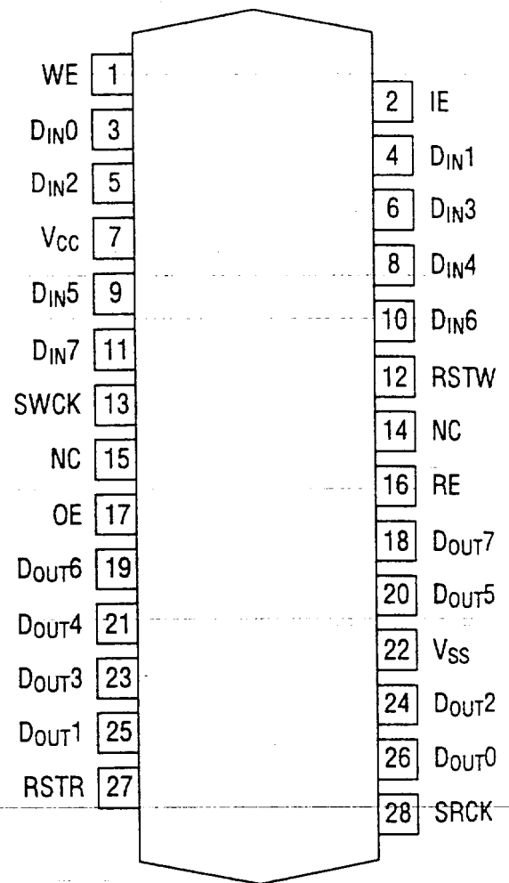
28-PIN ZIP
