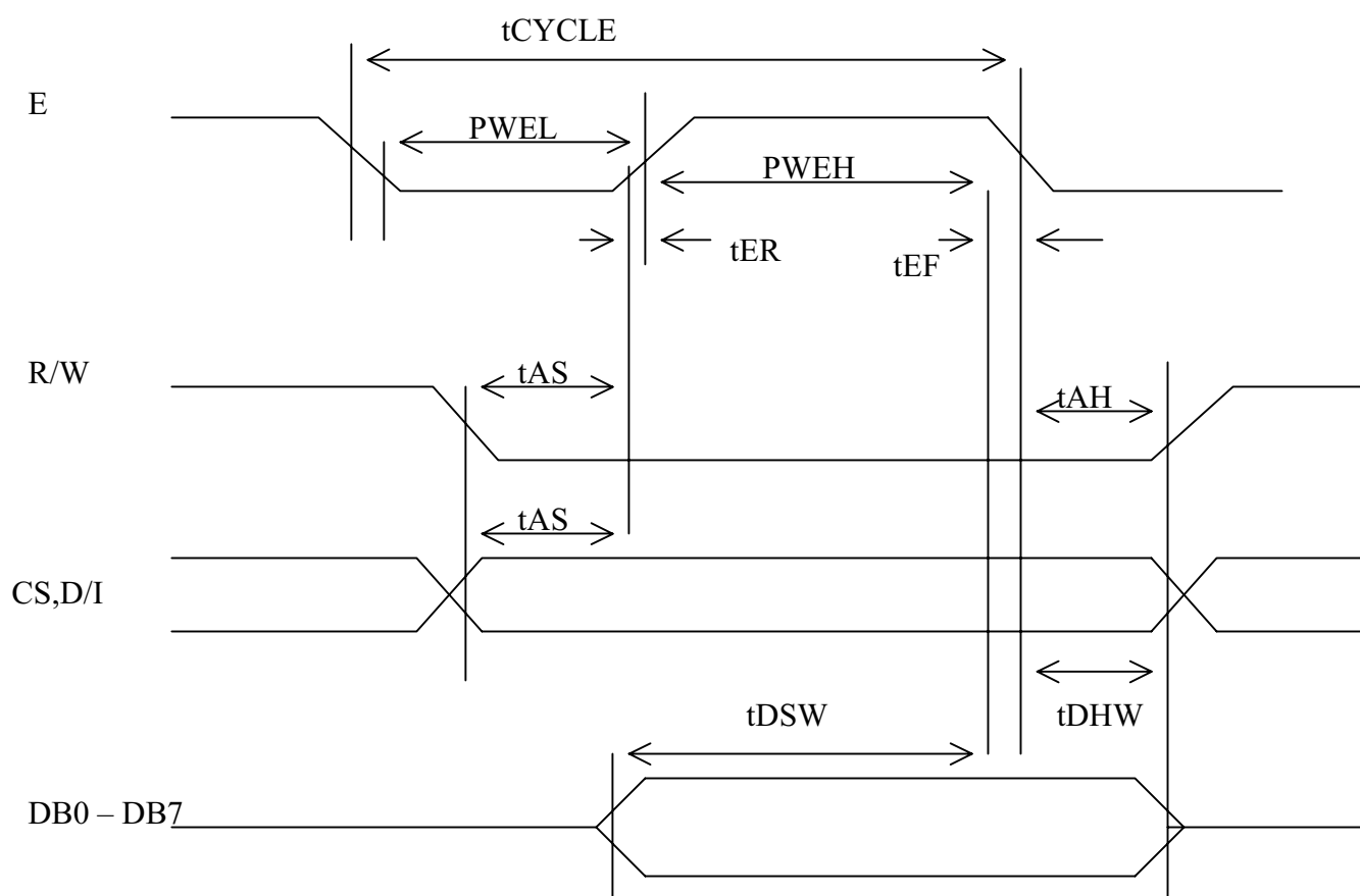
Write Timing Chart
