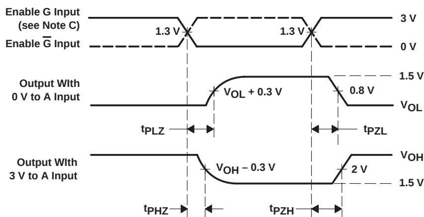
VOLTAGE WAVEFORMS
