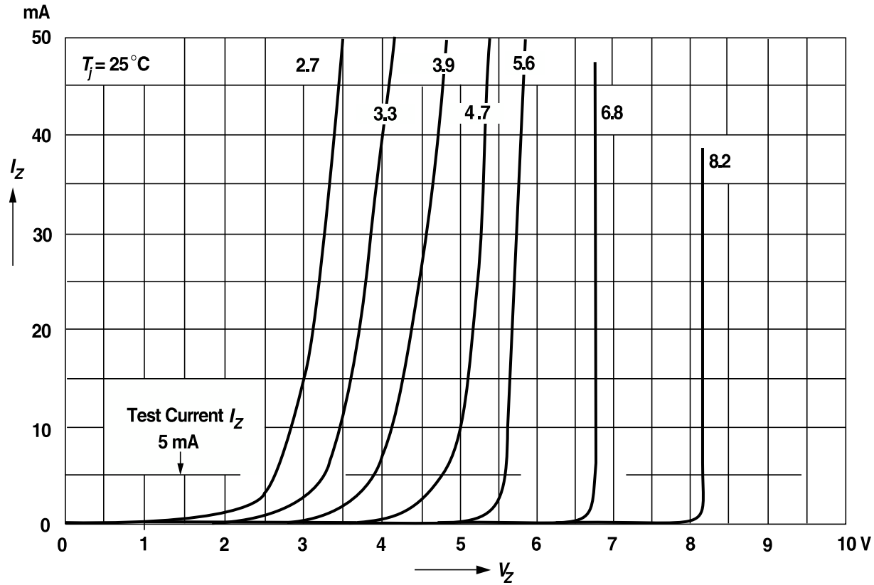
Figure 16. Breakdown Characteristics
