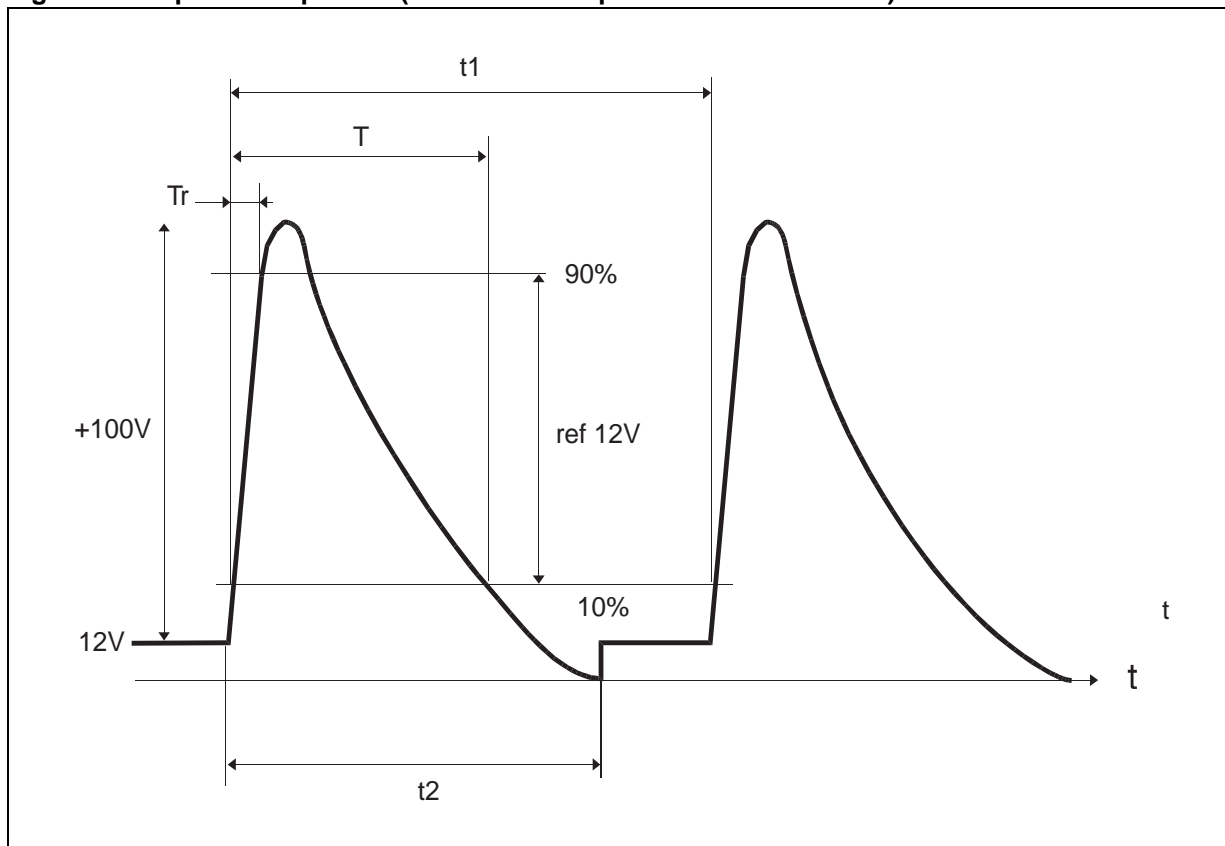
Figure 4. Shape of test pulse 2 (Sudden Interruption of Series Current)
