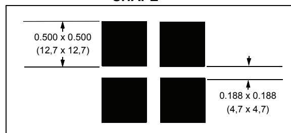
FIGURE 1: EXAMPLE PAD SIZES AND SHAPE
