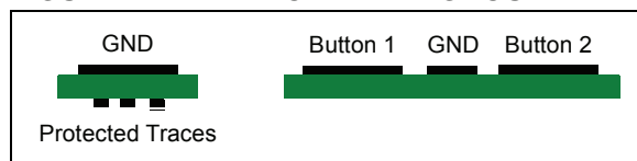
FIGURE 2: PROTECTIVE GROUND
