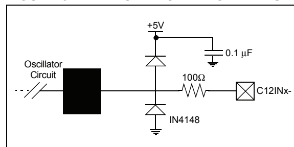
FIGURE 3: ESD PROTECTION CIRCUIT
