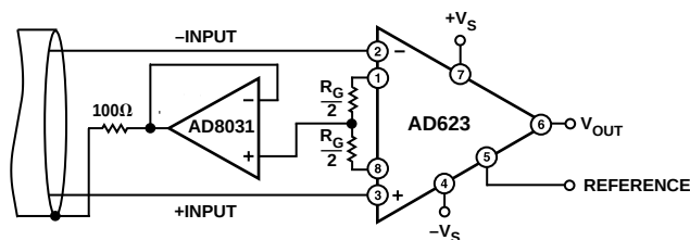
Figure 44. Common-Mode Shield Driver
