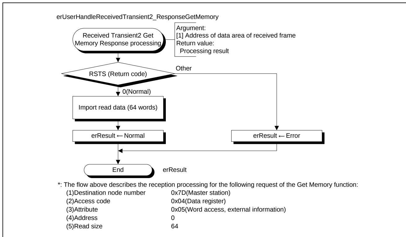
Figure 4.42 Received Transient2 Get Memory Response Processing Flowchart
