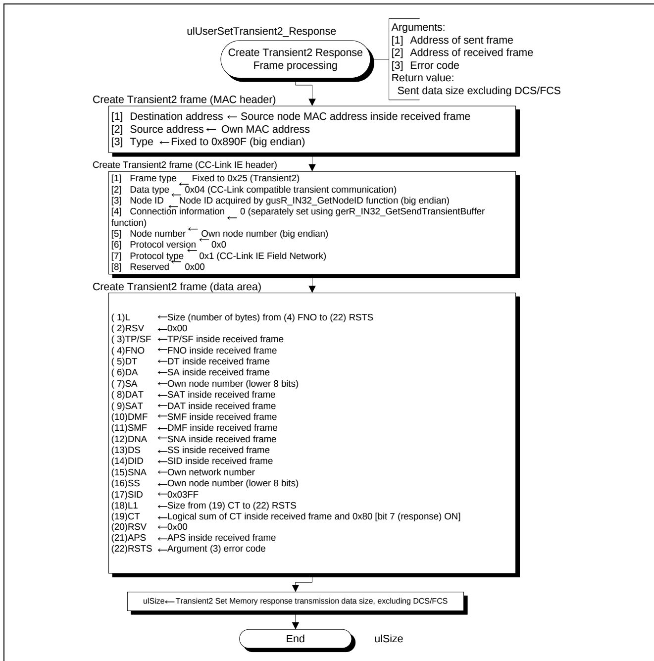
Figure 4.37 Create Transient2 Response Frame Processing Flowchart
