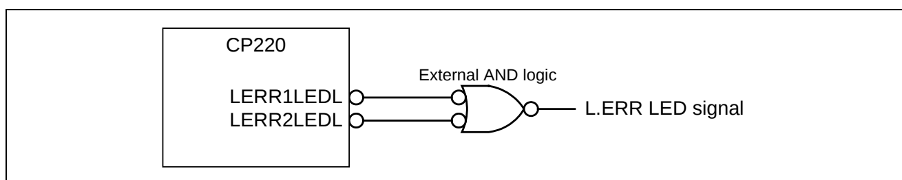
Figure 2.1 External AND Logic for Turning L.ERR On
