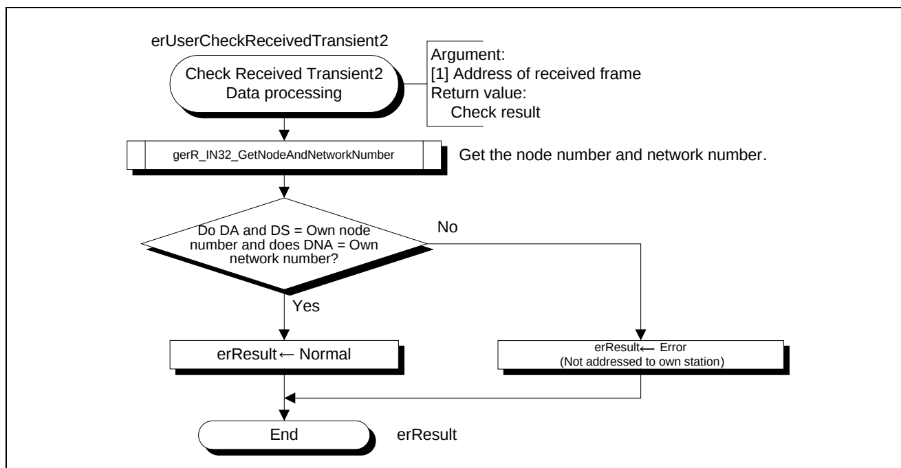
Figure 4.32 Check Received Transient2 Data Processing Flowchart
