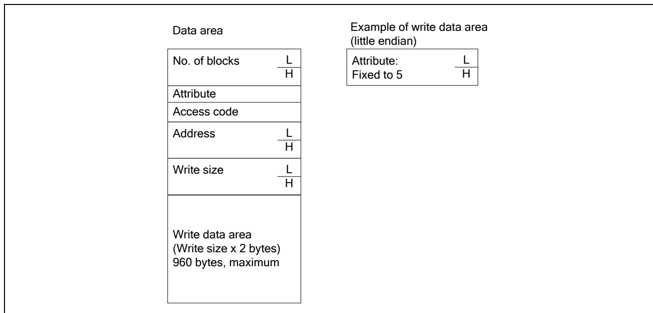
Figure 3.28 Set Memory Request
