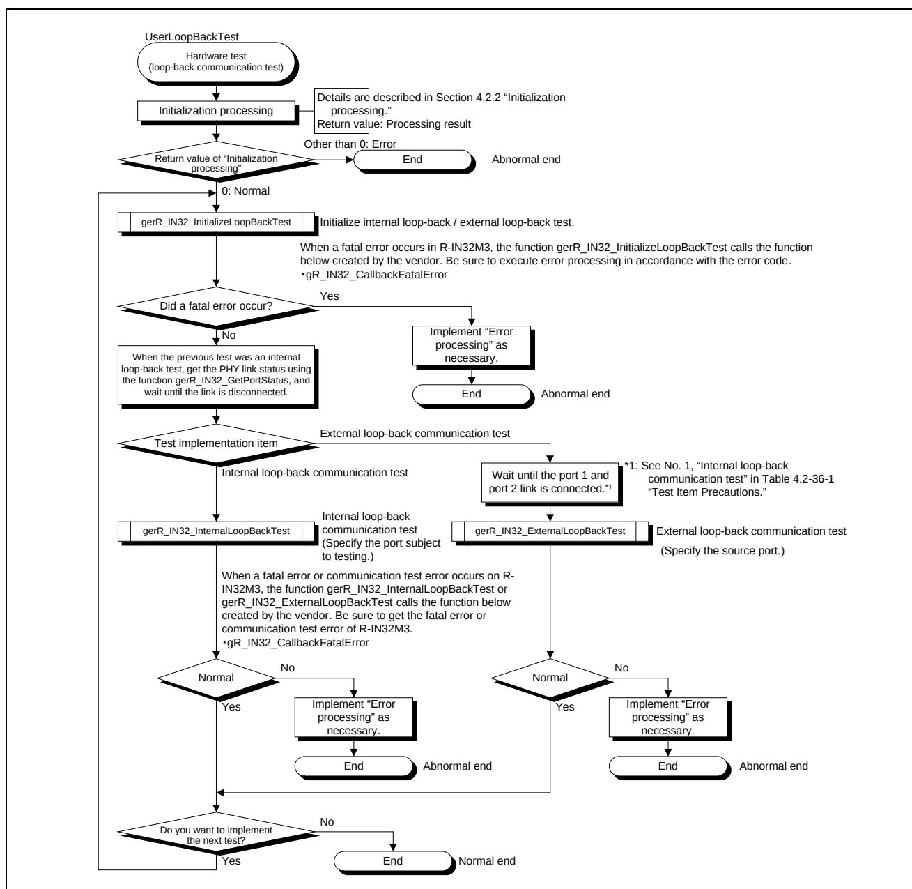
Figure 4.44 Hardware Test (Loop-back Communication Test) Flowchart
