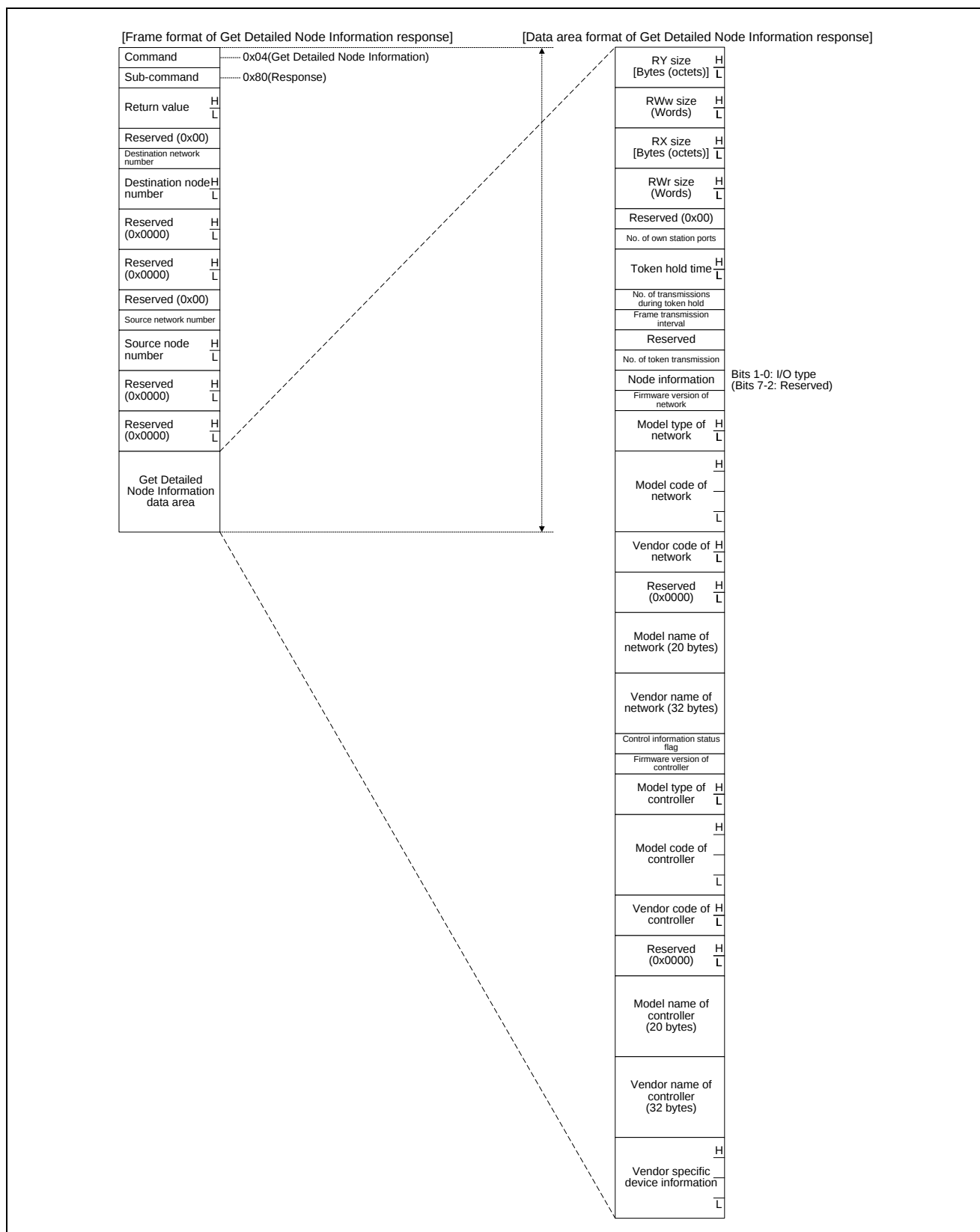
Figure 3.15 Transient1 Data Area: Get Detailed Node Information Response
