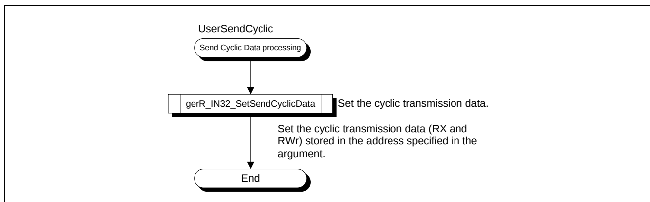
Figure 4.13 Send Cyclic Data Processing Flowchart
