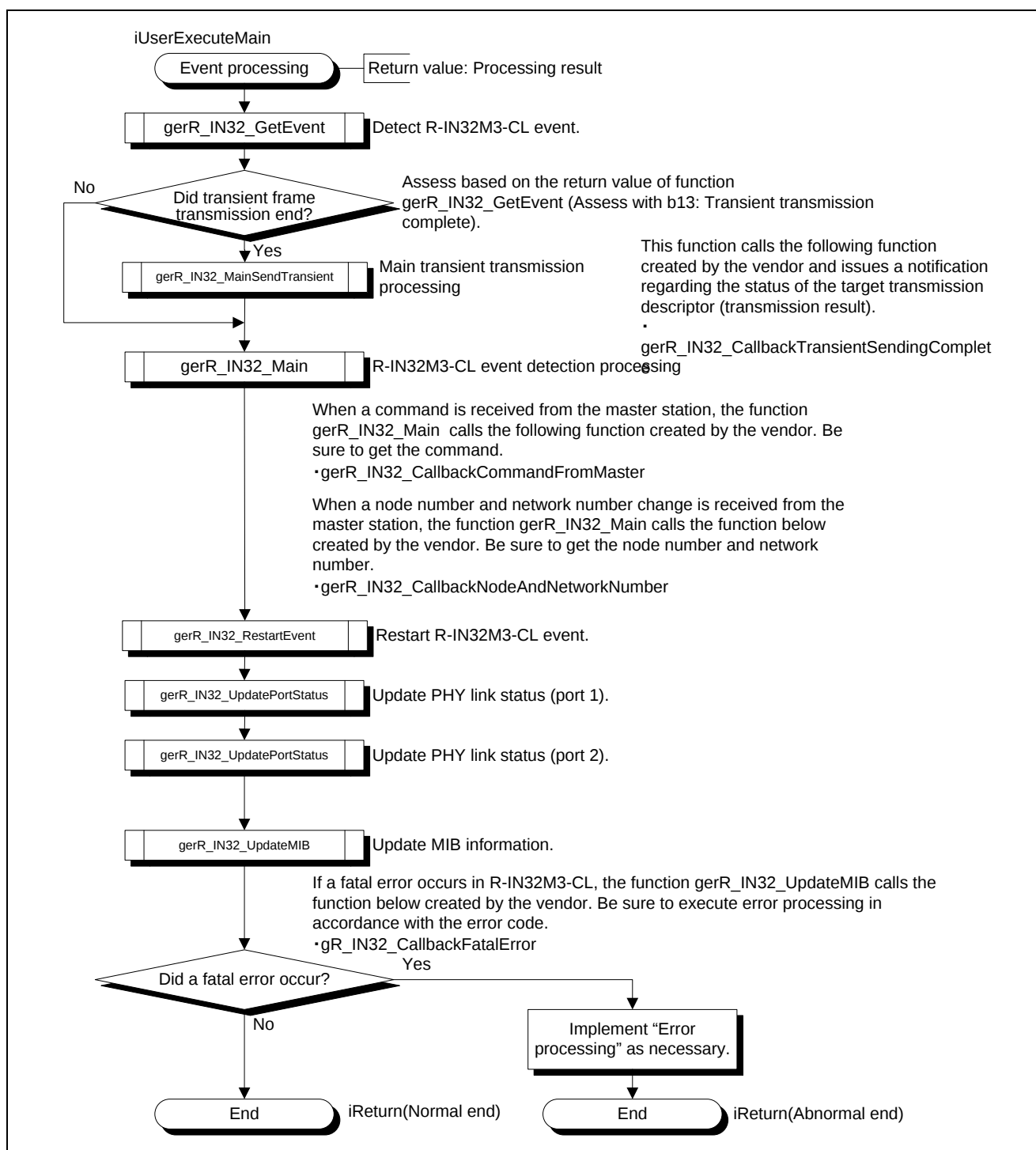
Figure 4.10 Event Processing Flowchart
