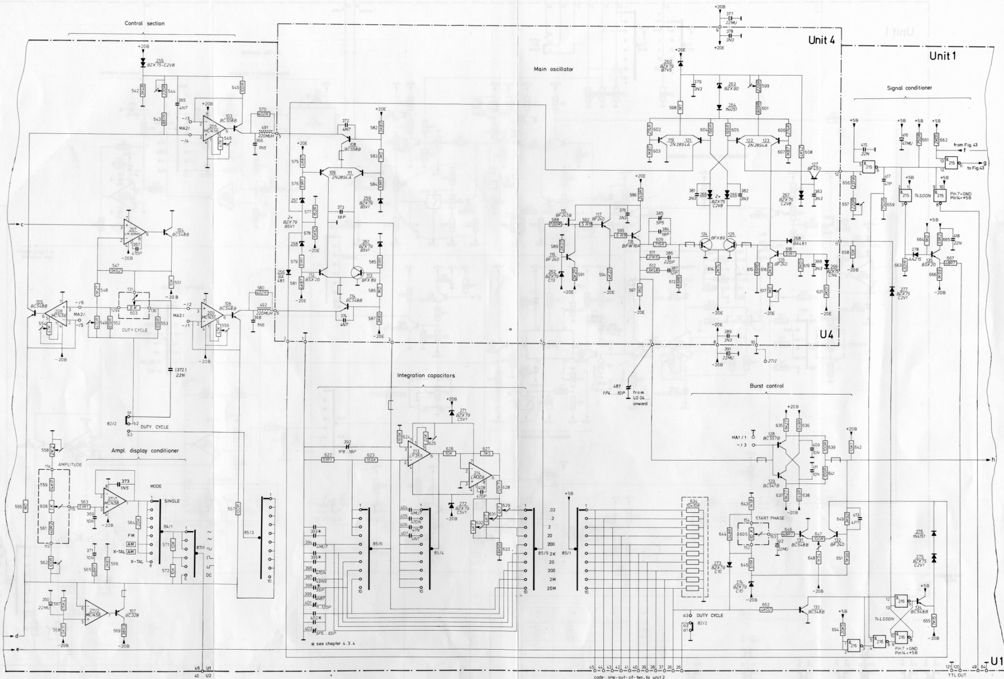
Fig. 42 Unit 1, part 2, circuit diagram
