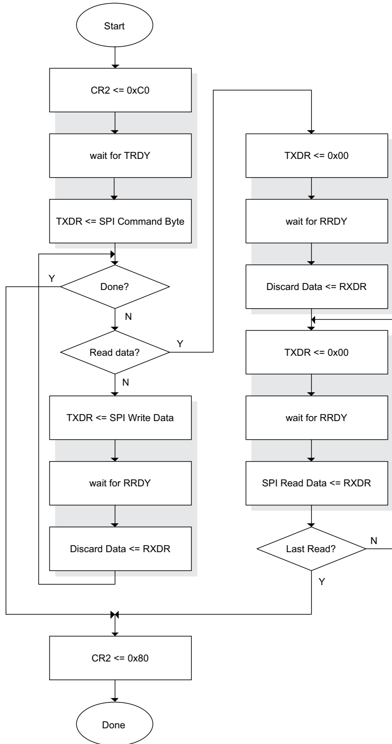
Figure 17-17. SPI Master Read/Write Example (via WISHBONE) – R1 Silicon
