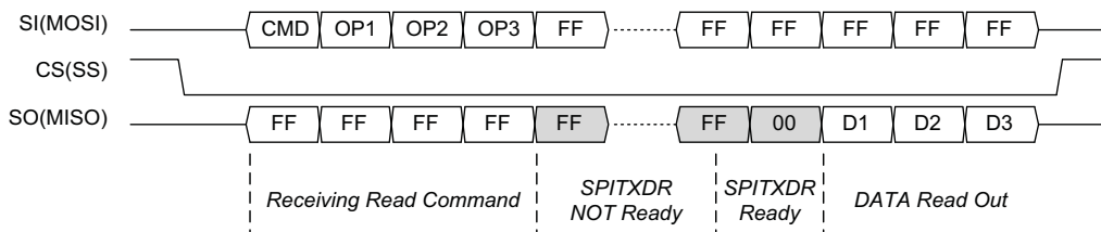
Figure 17-28. Slave SPI Dummy Byte Response (SPICR2[SDBRE]) Timing
