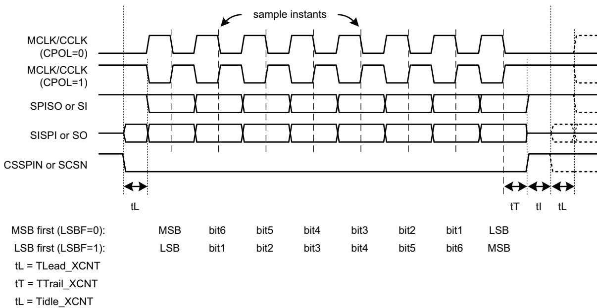
Figure 17-25. SPI Control Timing (SPICR2[CPHA]=1, SPICR1[TXEDGE]=0)
