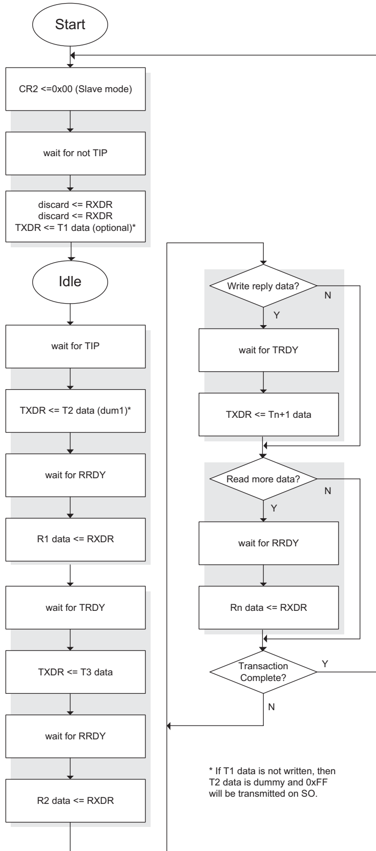
Figure 17-18. SPI Slave Read/Write Example (via WISHBONE) - Production Silicon
