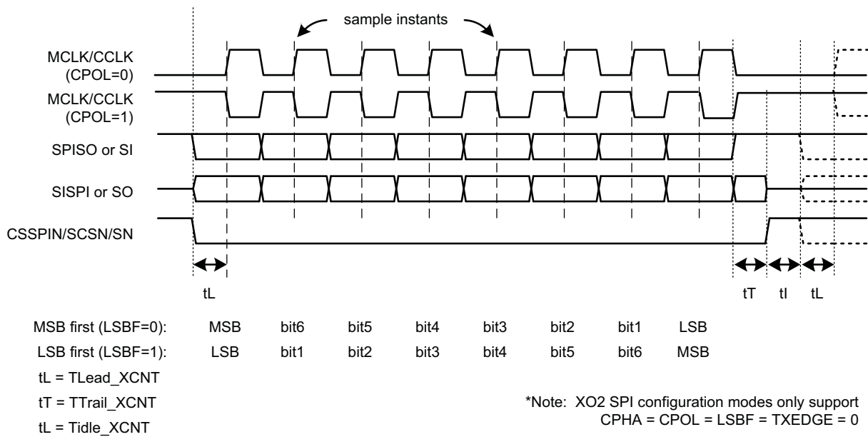
Figure 17-24. SPI Control Timing (SPICR2[CPHA]=0, SPICR1[TXEDGE]=0)
