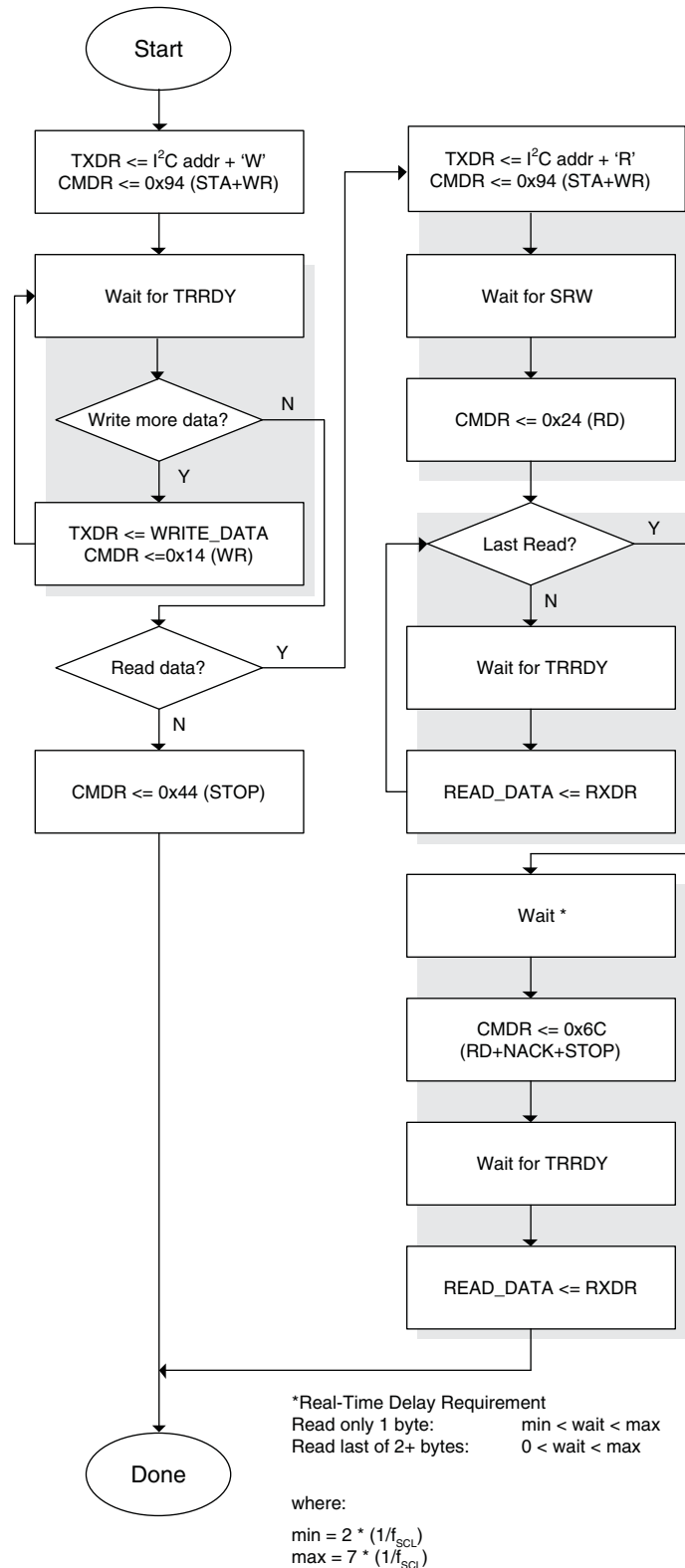
Figure 17-6. I 2 C Master Read/Write Example (via WISHBONE)
