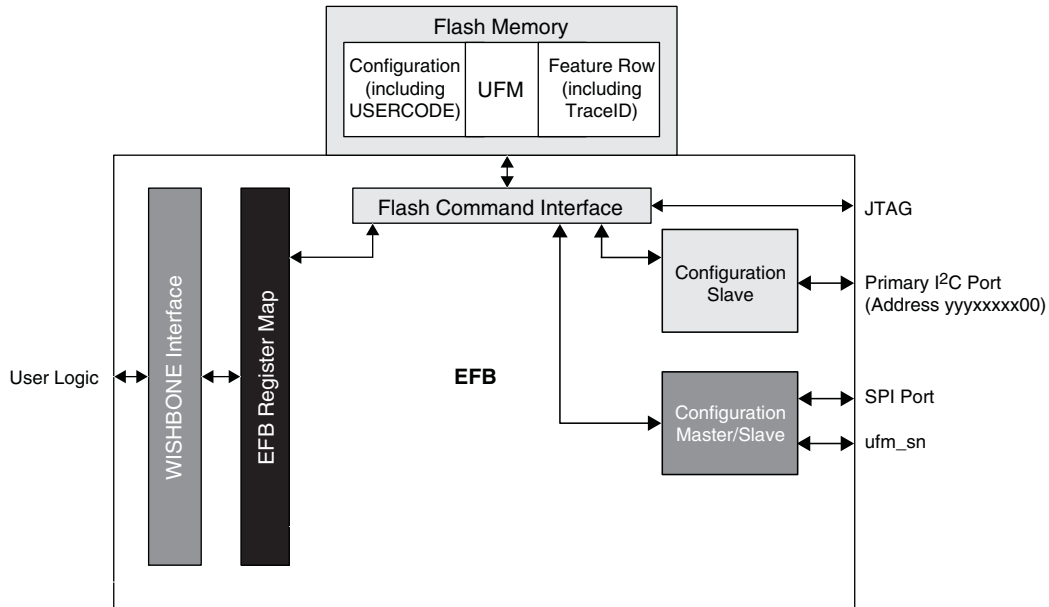
Figure 17-29. Interfaces to the UFM/Configuration Sectors
