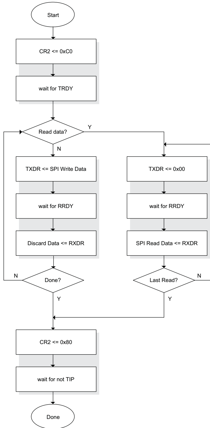
Figure 17-16. SPI Master Read/Write Example (via WISHBONE) – Production Silicon
