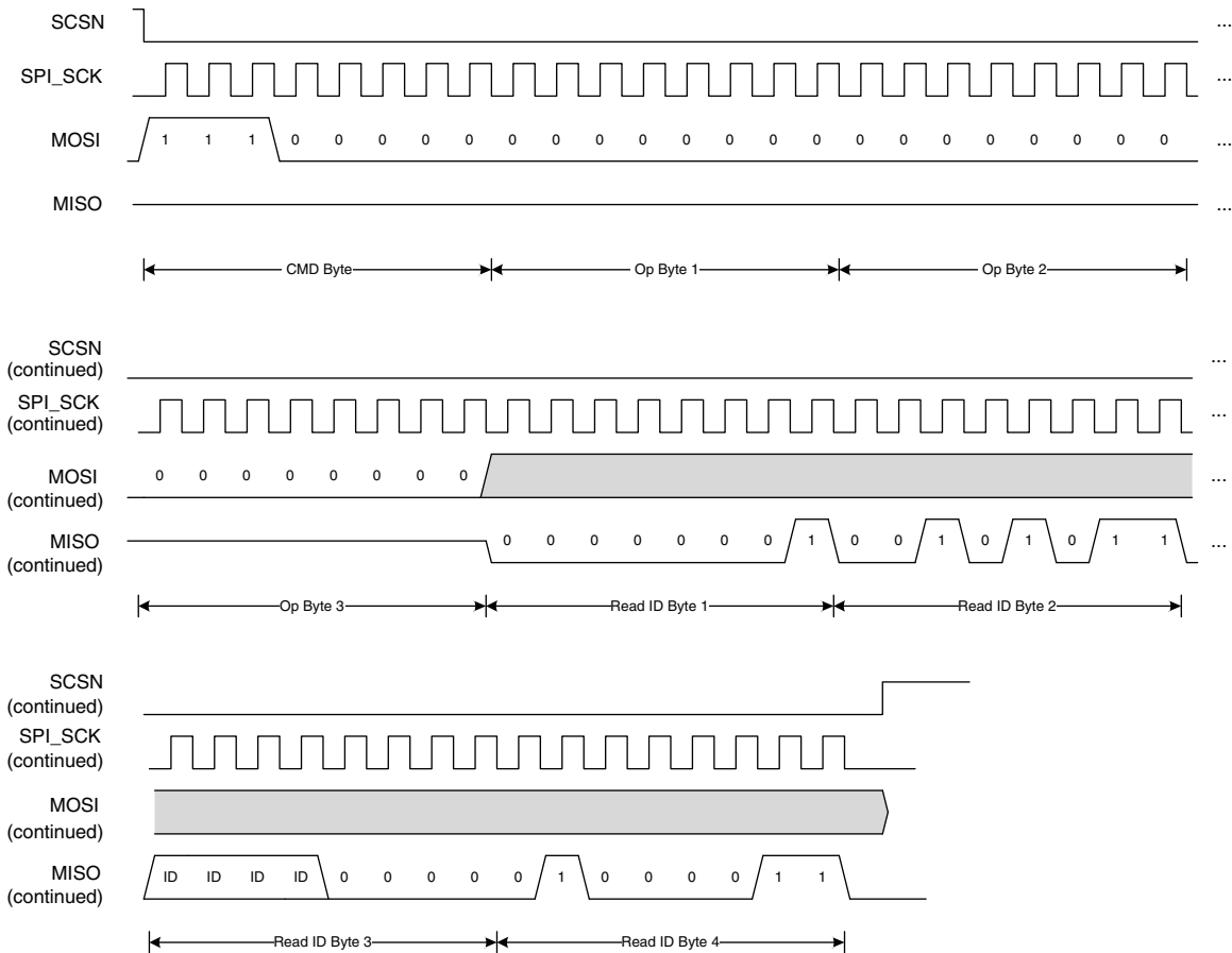
Figure 17-33. SSPI Read Device ID Example
