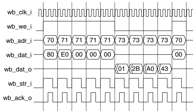
Figure 17-34. WISHBONE Read Device ID Example (-1200 HC Device)
