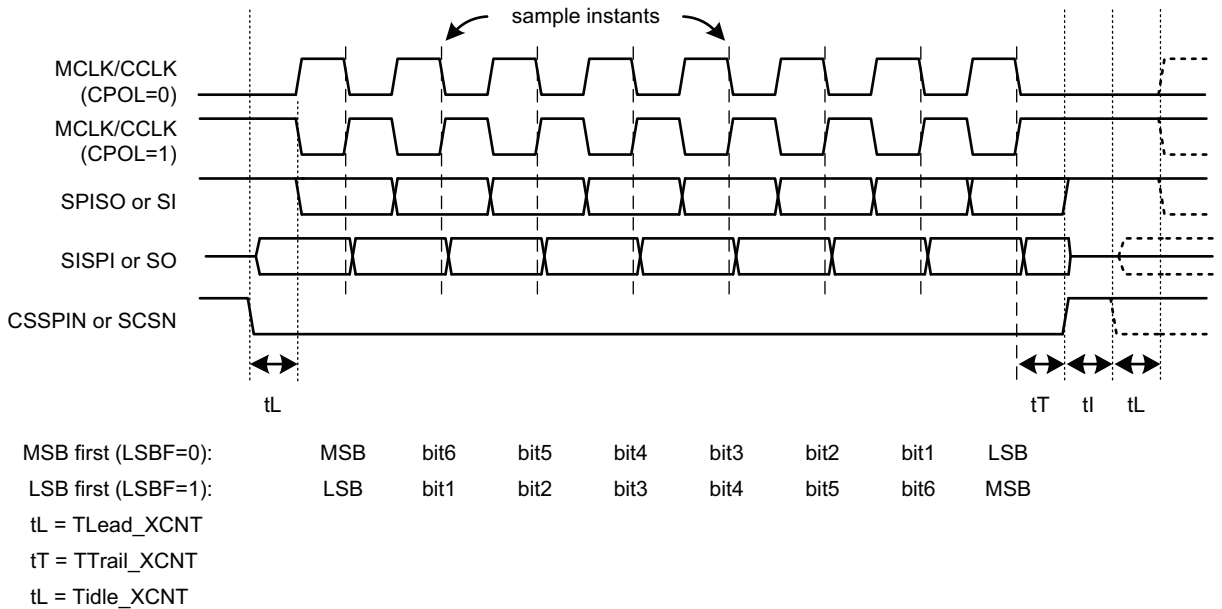
Figure 17-28. Slave SPI Dummy Byte Response (SPICR2[SDBRE]) Timing
