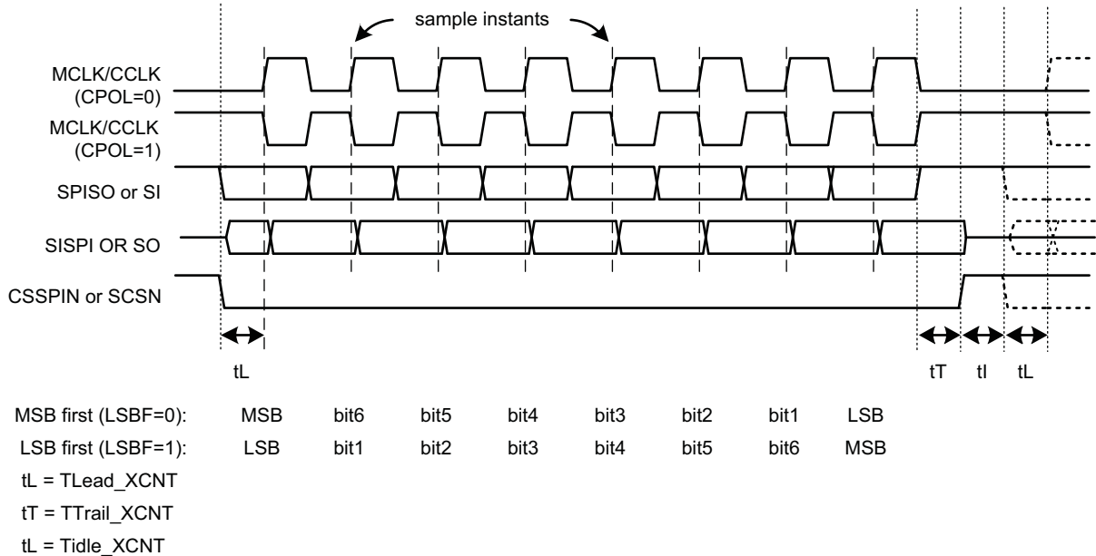
Figure 17-27. SPI Control Timing (SPICR2[CPHA]=1, SPICR1[TXEDGE]=1)
