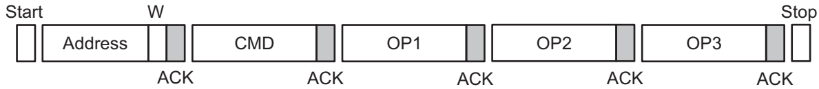
Figure 17-9. I 2 C Command with Write Data (e.g. LSC_PROG_INCR_NV)
