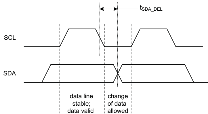
Figure 17-15. I 2 C Bit Transfer Timing
