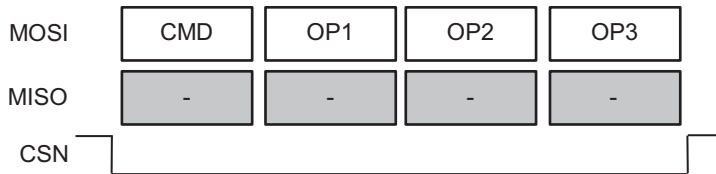
Figure 17-20. SPI Command w/ Write Data (e.g. LSC_PROG_INCR_NV)
