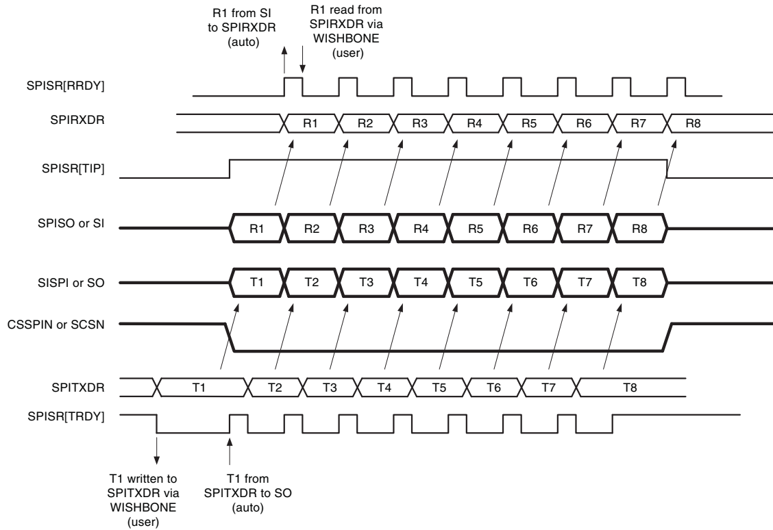
Figure 17-23. Minimally Specified SPI Transaction Example (MachXO2 as SPI Slave)
