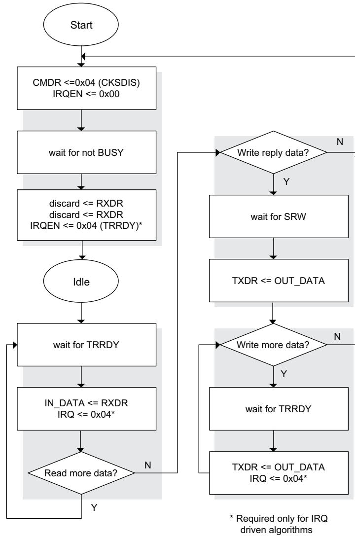
Figure 17-7. I 2 C Slave Read/Write Example (via WISHBONE)
