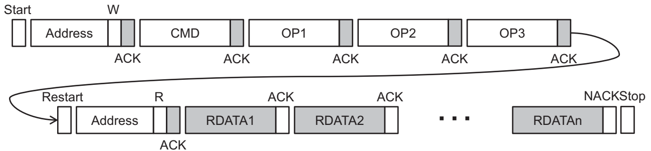
Figure 17-10. I 2 C Command with Read Data (e.g. LSC_READ_STATUS)
