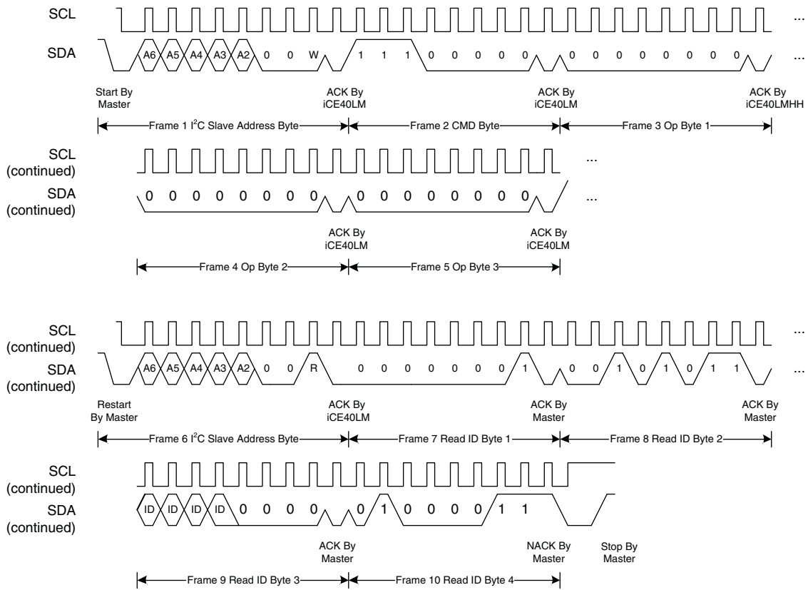
Figure 17-32. I 2 C Read Device ID Example
