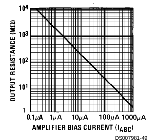
Output Resistance
