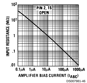
Input Resistance
