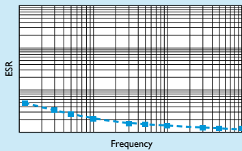
Fig. I-10 ESR Change vs. Frequency
