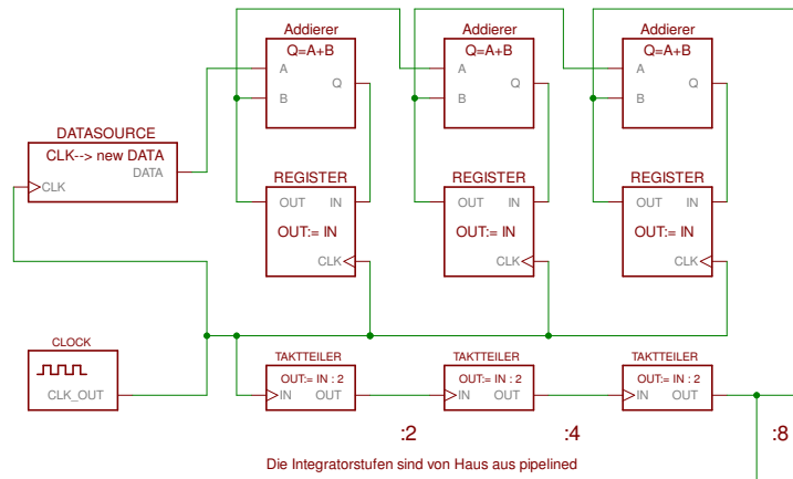
Integrator, 3 Stufen
