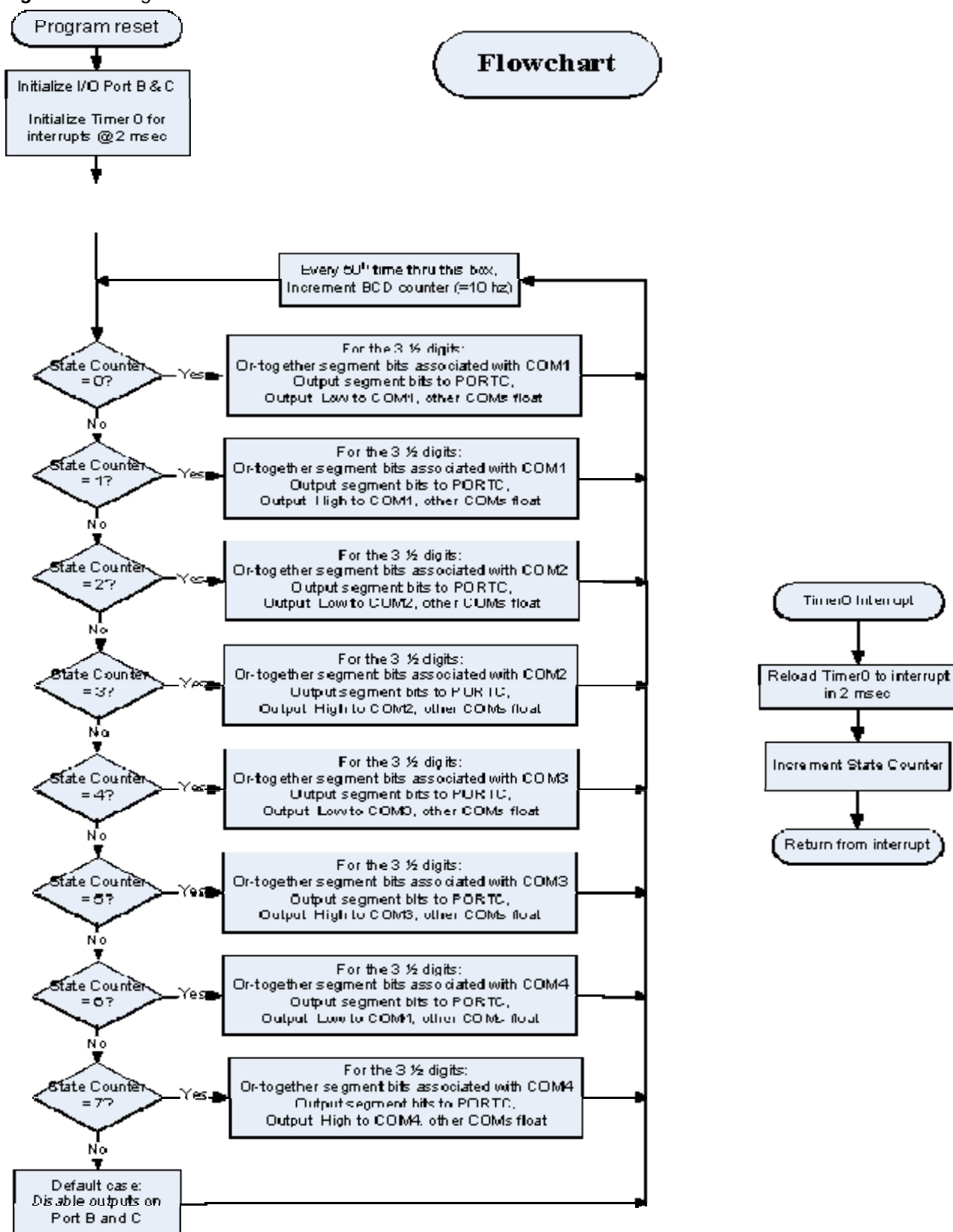
Figure 3-2. Program flowchart.
