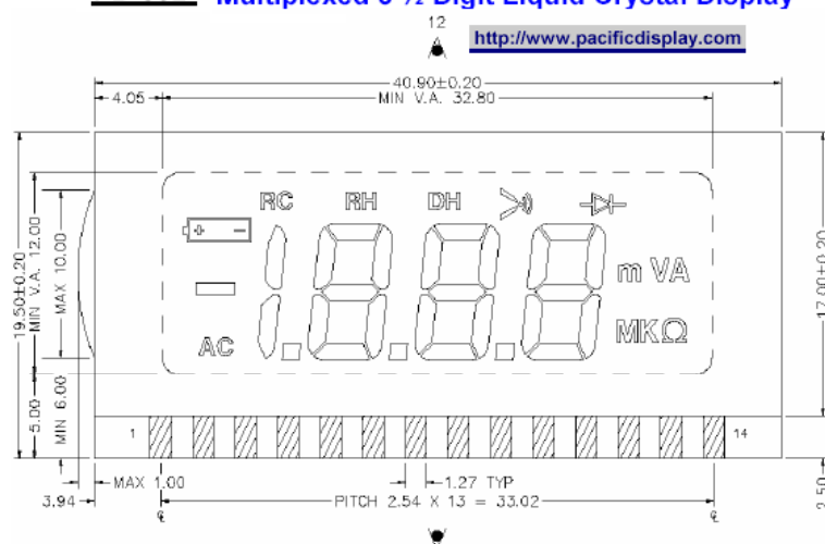
Figure 2-1. LCD footprint
