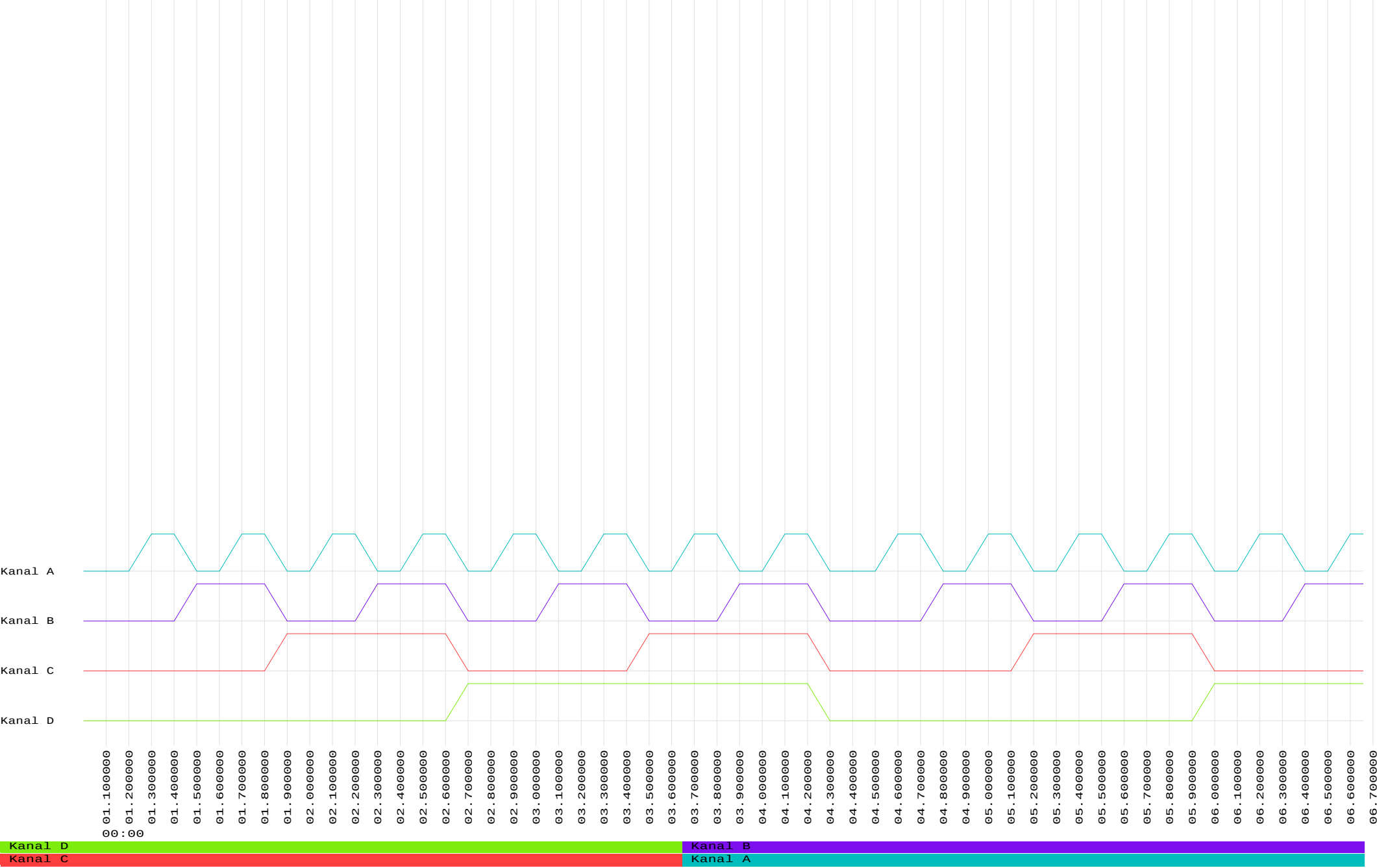
zaehler.csv
