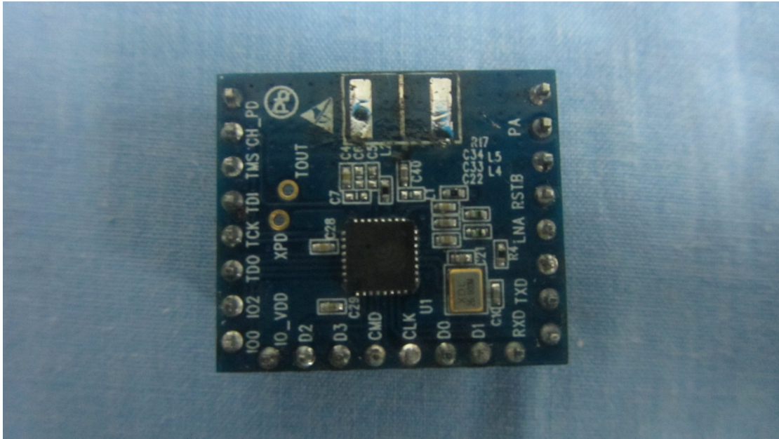
ESP8266EX Internal Photo
