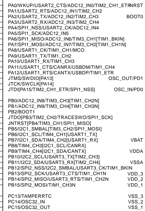
U2 STM32F103C8T6
