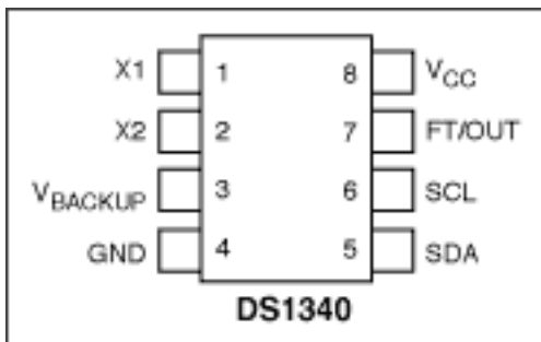
Pin Assignment
