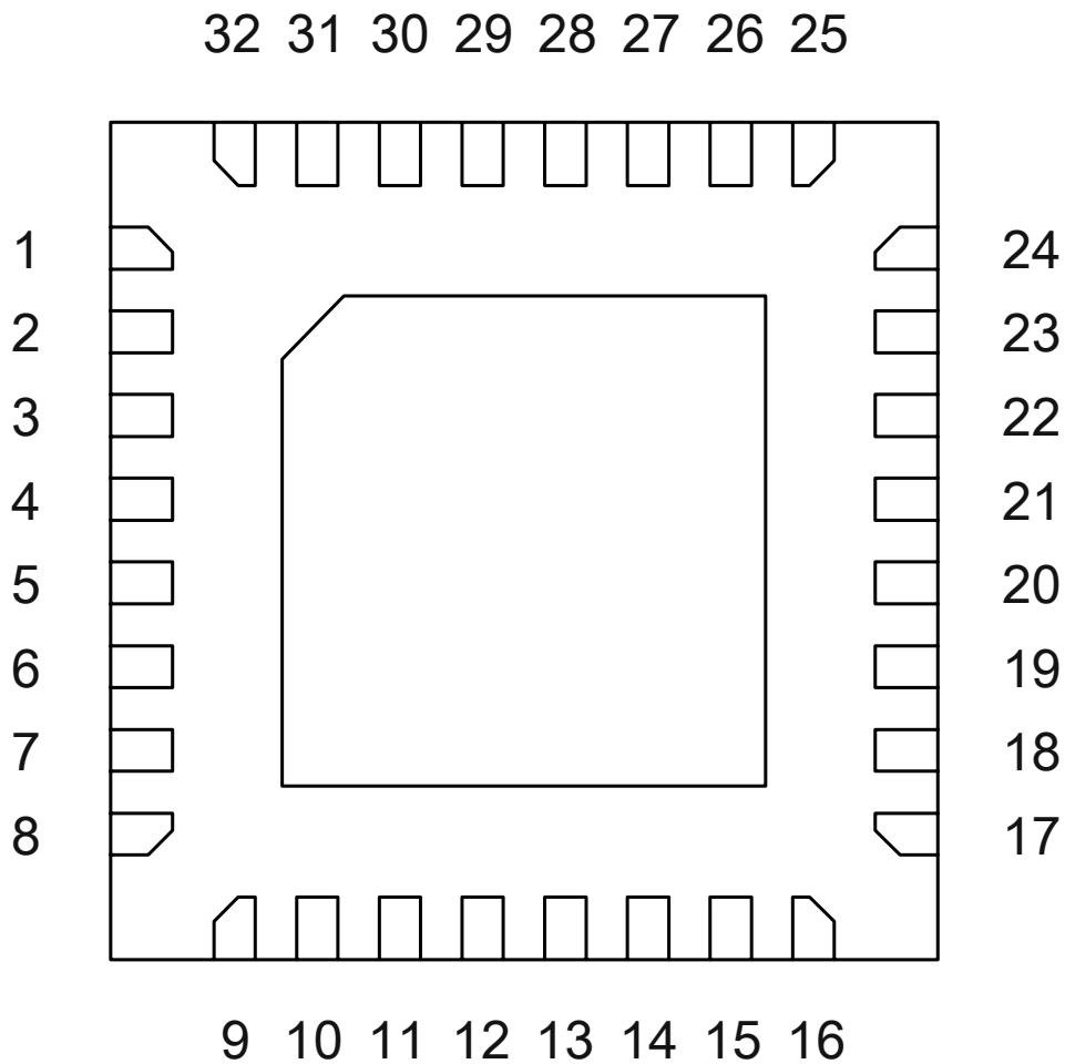
Figure 1.1: Pinout Diagram
