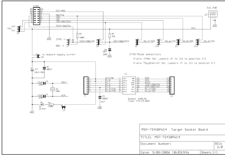
Figure B-3. MSP-TS430PW14 Target Socket Module, Schematic
