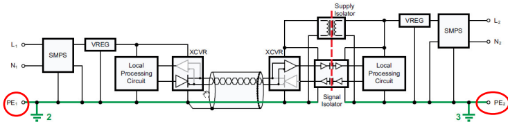
Figure 10. Isolation of Two Remote Transceiver Stations With Single-Ground Reference
