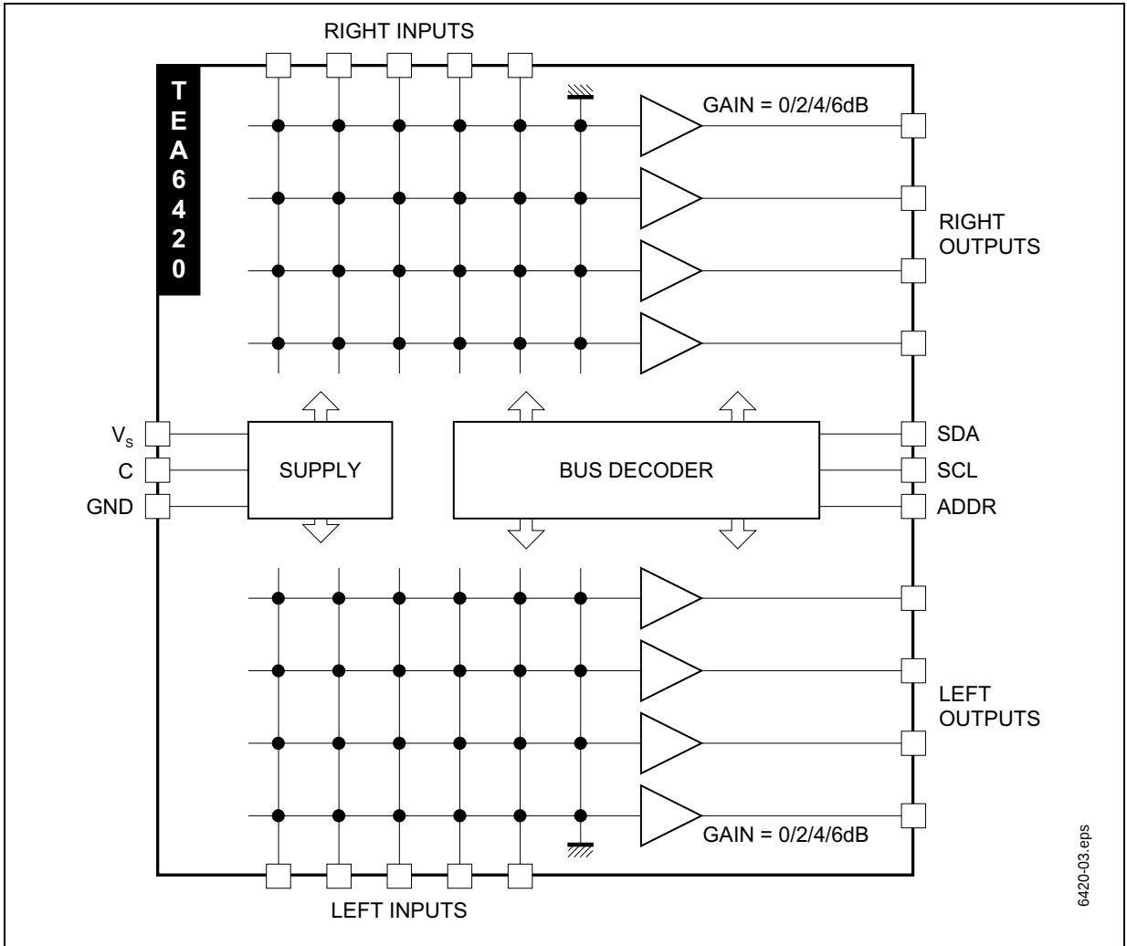
Figure 2. BLOCK DIAGRAM
