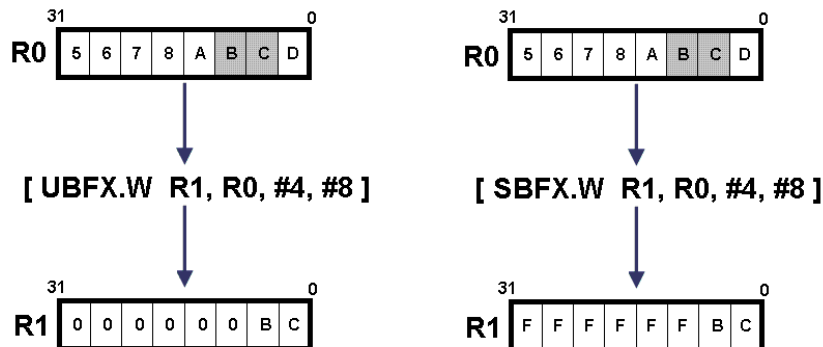
Figure 13. Bit extraction with the UBFX and SBFX instructions
