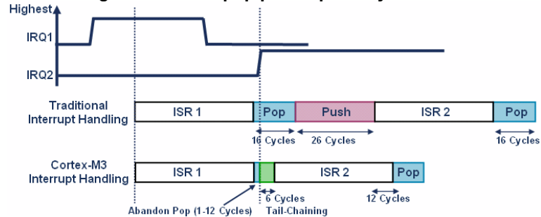
Figure 12. Stack pop pre-emption by the NVIC
