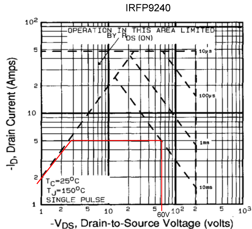
Fig 8. Maximum Safe Operating Area
