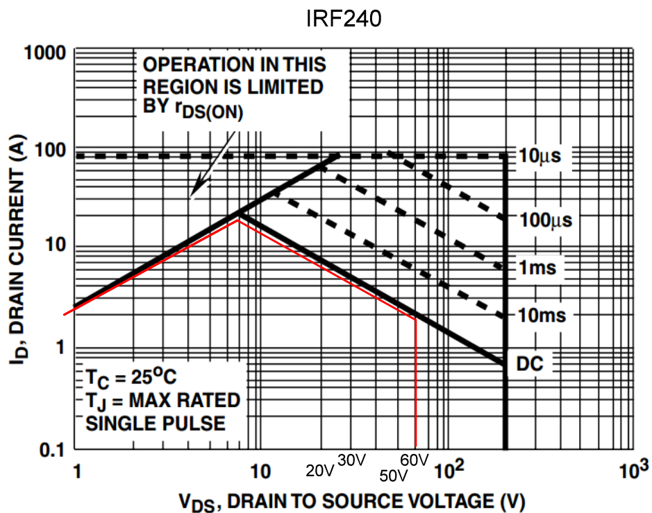
FIGURE 4. FORWARD BIAS SAFE OPERATING AREA
