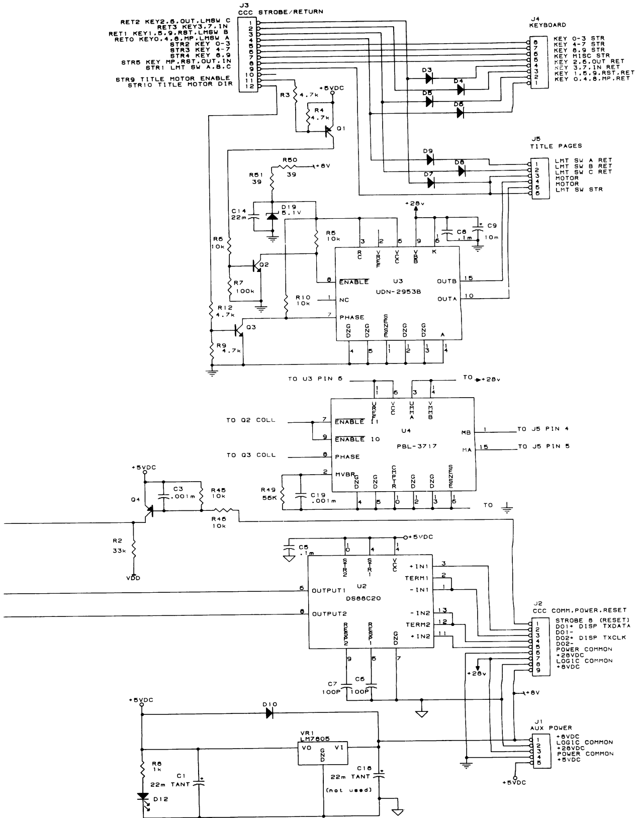
Figure 5-11. Display Assembly
