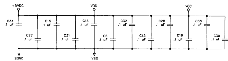
Figure 5-12A. Central Control Computer Schematic, Sheet 1
