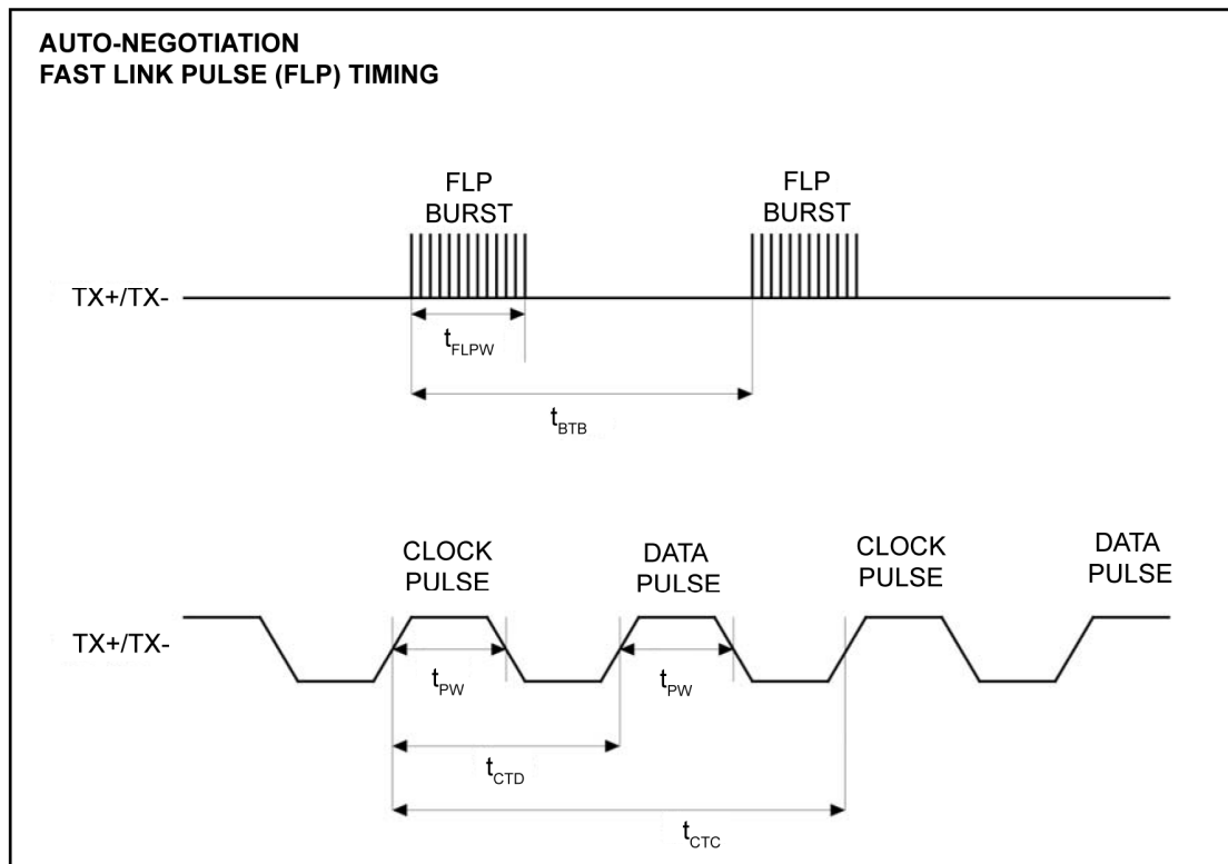
Figure 18. Auto-Negotiation Fast Link Pulse (FLP) Timing
