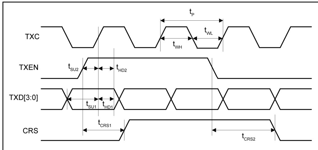
Figure 14. MII Transmit Timing (10Base-T)
