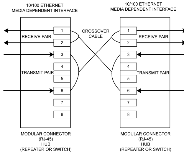
Figure 8. Typical Crossover Cable Connection
