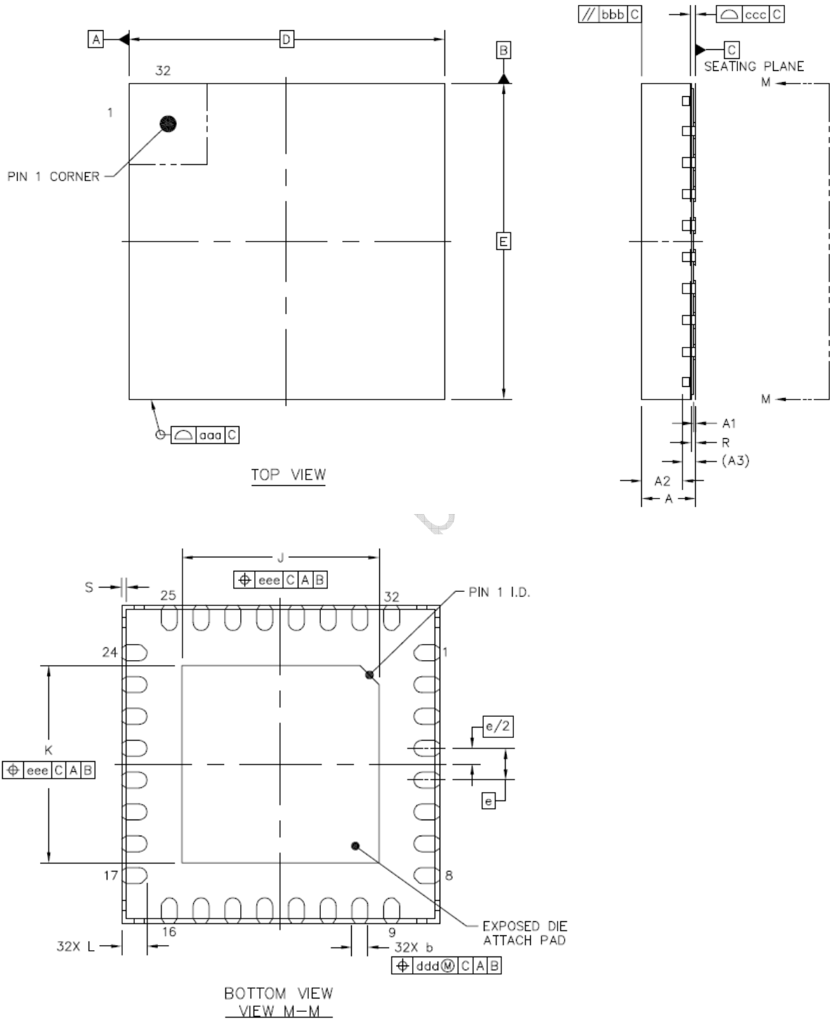
32-Pin (5mm x 5mm) WQFN
