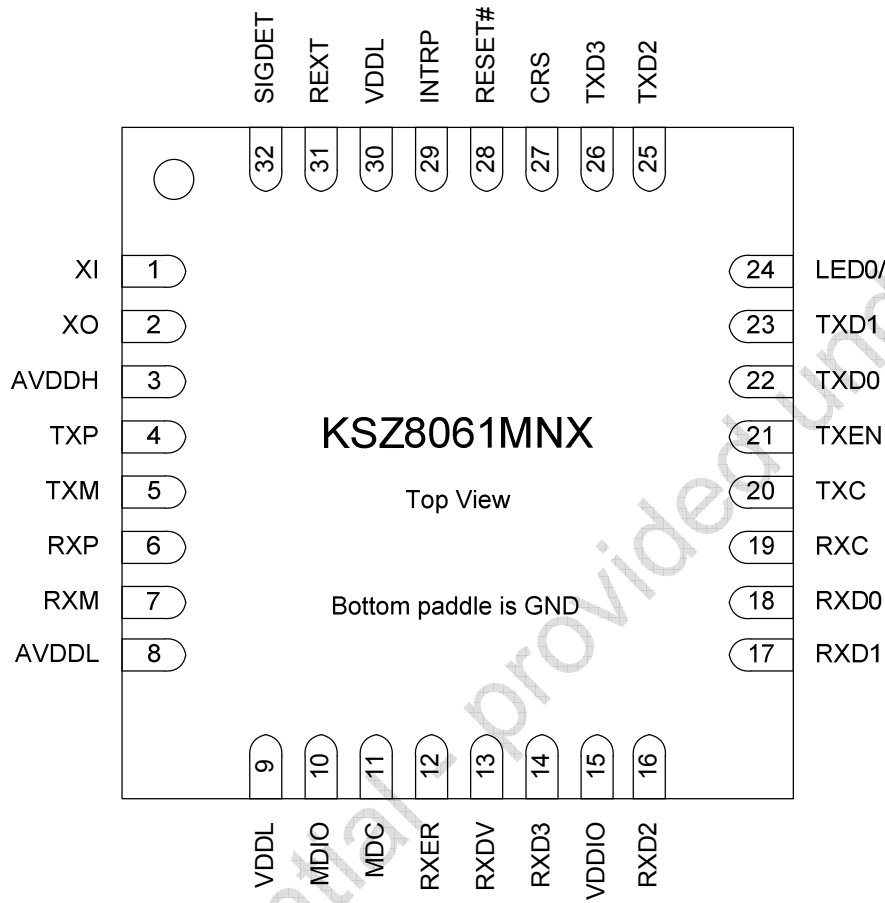
Figure 1 KSZ8061MNX Pinout
