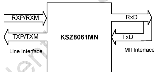
Figure 6. KSZ8061MN Back-to-Back for MII Bus Loopback
