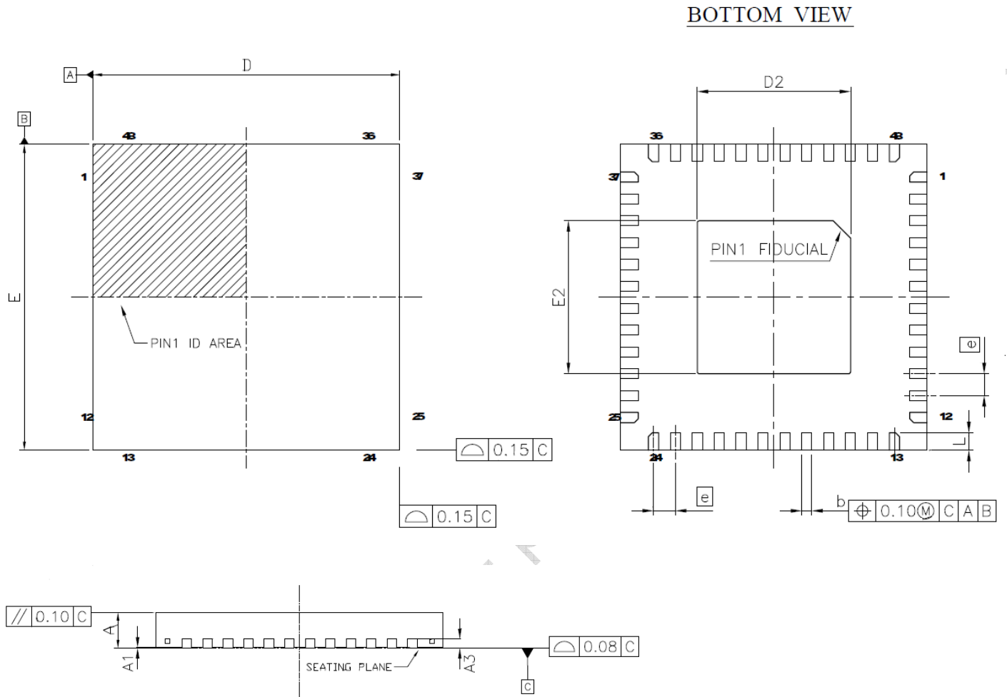
48-Lead (7mm x 7mm) QFN
