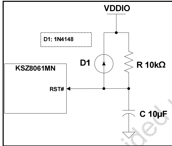
Figure 21. Recommended Reset Circuit
