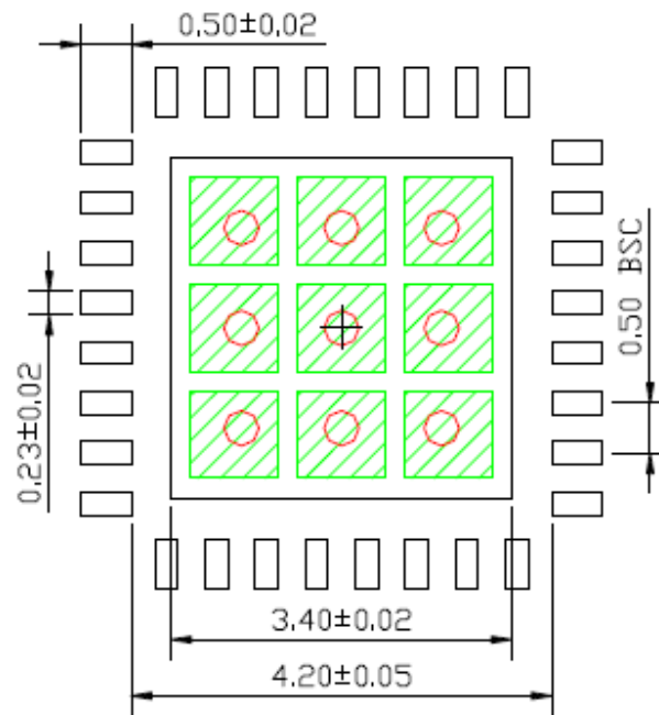
Figure 24 Land Pattern for WQFN-32LD and QFN-32LD
