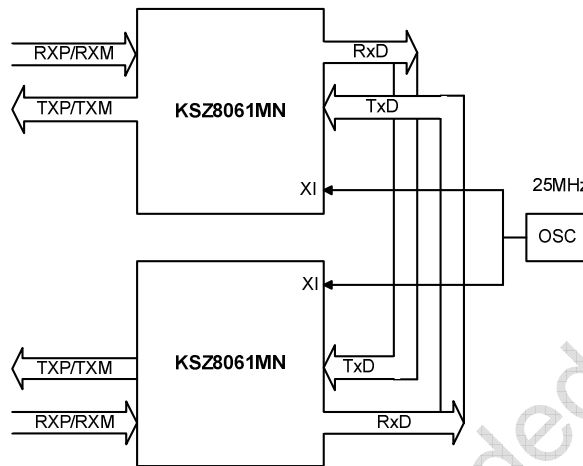
Figure 5. KSZ8061MN to KSZ8061MN Back-to-Back Repeater
