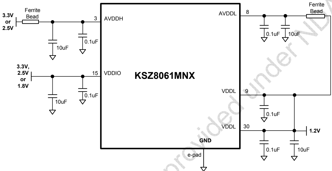
Figure 12. KSZ8061MNX Power and Ground Connections
