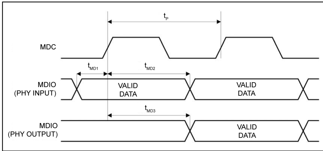
Figure 19. MDC/MDIO Timing
