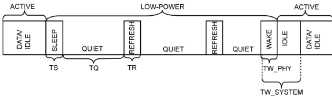
Figure 11. LPI Mode (Refresh Transmissions and Quiet Periods)
