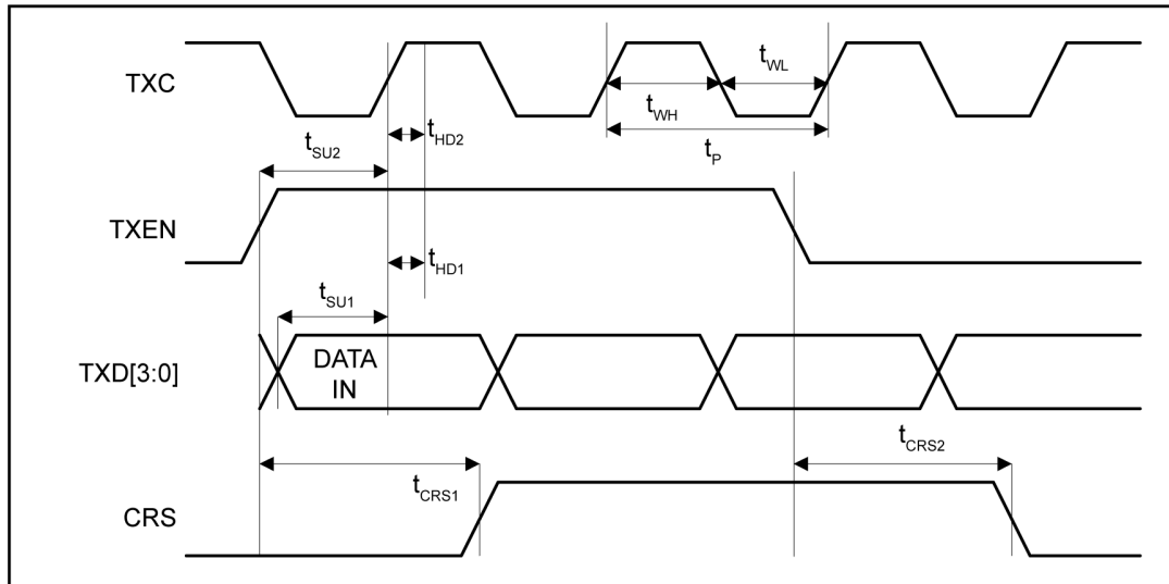
Figure 16. MII Transmit Timing (100Base-TX)
