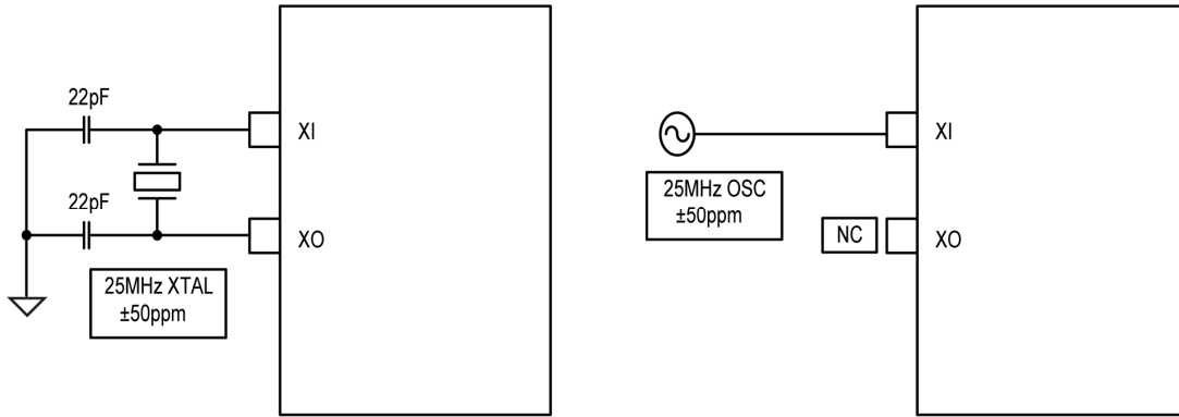
Figure 23. 25MHz Crystal / Oscillator Reference Clock Connection
