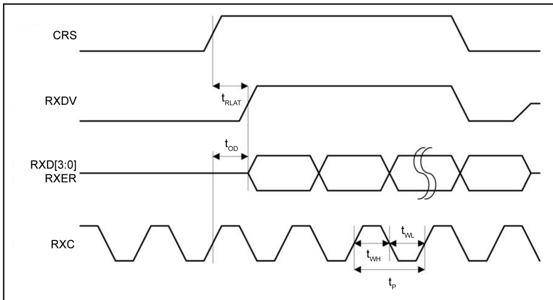
Figure 17. MII Receive Timing (100Base-TX)
