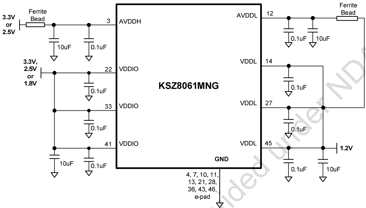
Figure 13. KSZ8061MNG Power and Ground Connections
