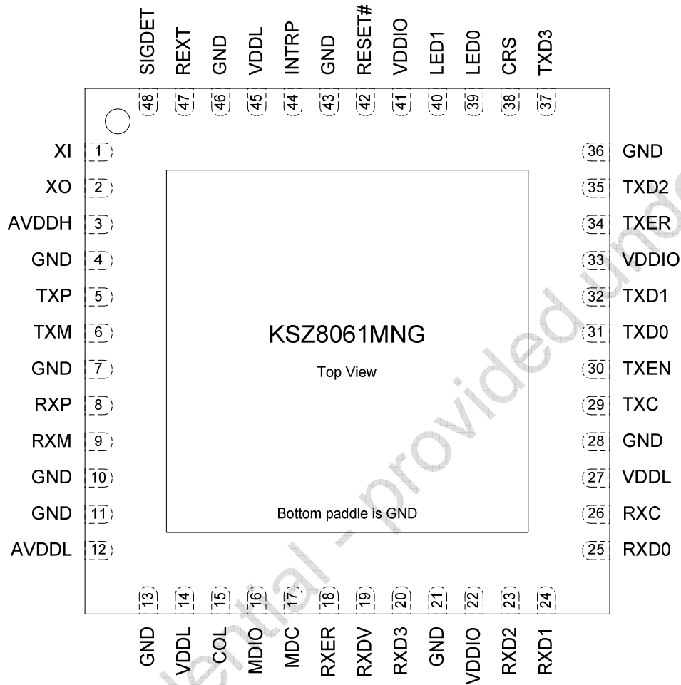
Figure 2 KSZ8061MNG Pinout
