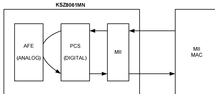
Figure 9. Local (Digital) Loopback
