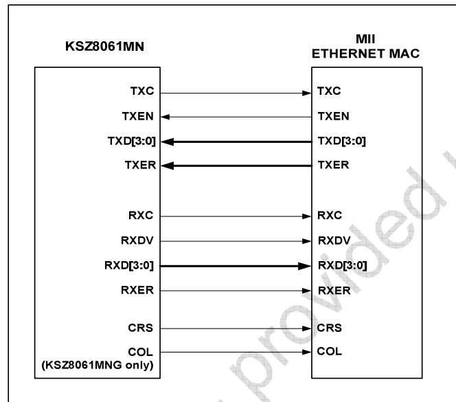
Figure 4. KSZ8061MN MII Interface
