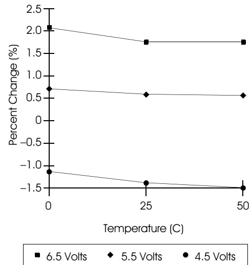
Graph 2-32: Oscillator Stability
