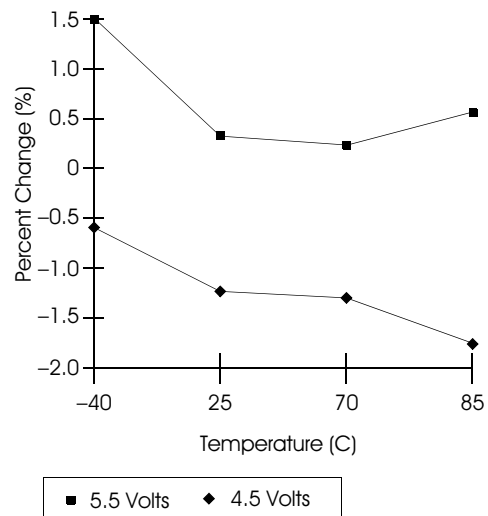
Graph 2-28: Oscillator Stability
