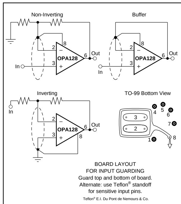
FIGURE 2. Connection of Input Guard.
