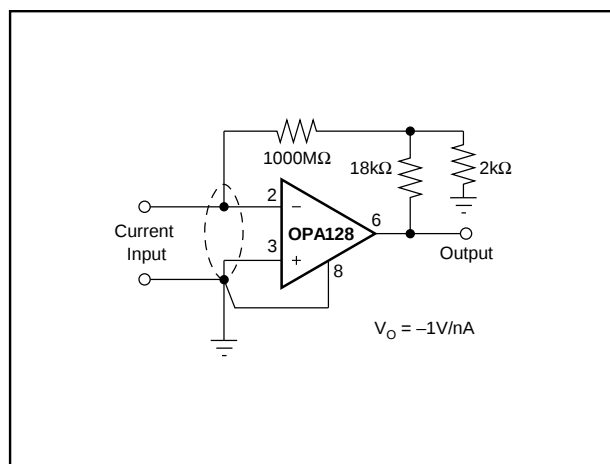
FIGURE 8. Current-to-Voltage Converter.
