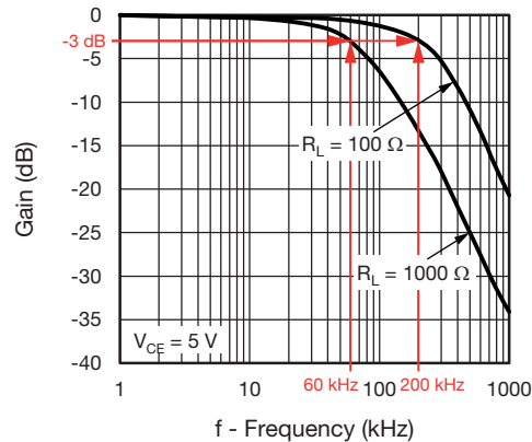
Fig. 16 - Gain vs. Frequency
