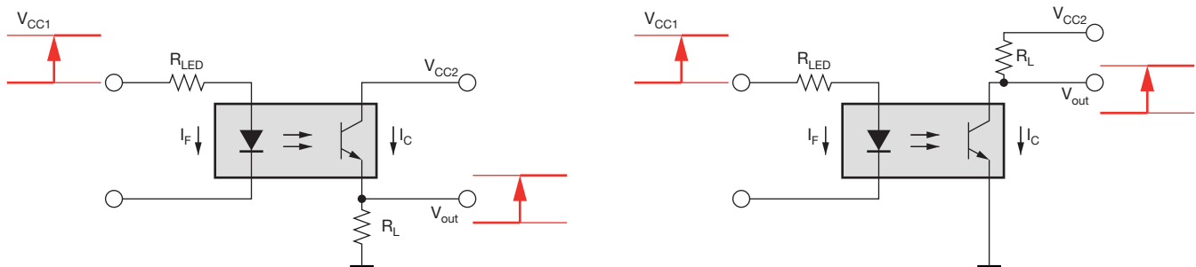
Fig. 13 - Optocoupler in Common Collector C-C (left) and Common Emitter C-E (right) Configurations
