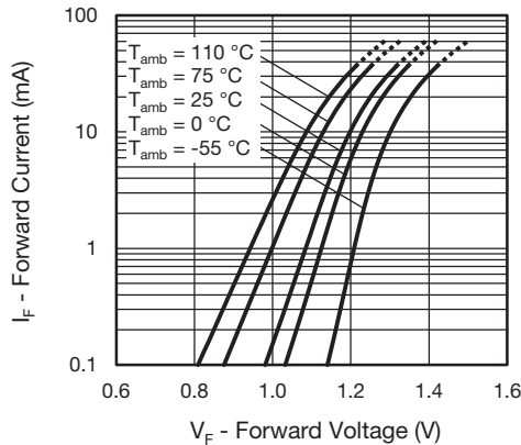
Fig. 10 - Emitter Diode Forward Current vs. Forward Voltage
