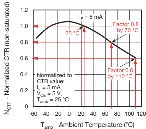
Fig. 14 - Normalized CTR (non-saturated) vs. Ambient Temperature
