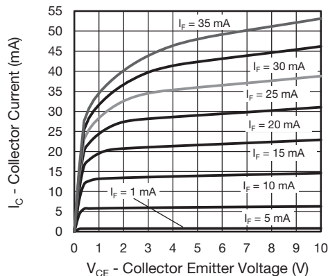
Fig. 11 - Collector Current vs. Collector Emitter Voltage (non-saturated)
