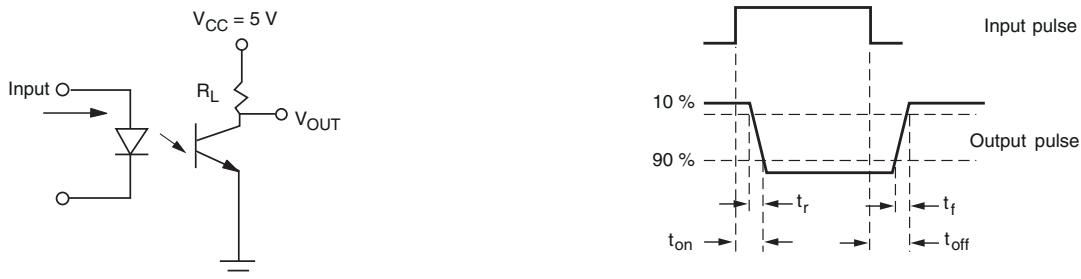
Fig. 8 - Test Circuit and Switching Waveforms
