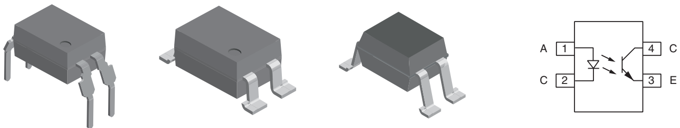
Fig. 2 - Typical Packages and Symbols
