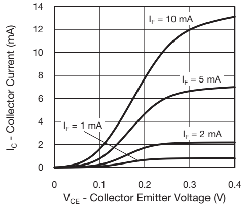
Fig. 12 - Collector Current vs. Collector-Emitter Voltage (saturated)
