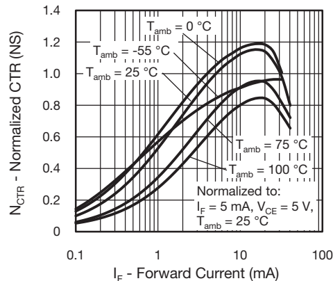
Fig. 15 - Normalized CTR (non-saturated) vs. Forward Current ( I_F )
