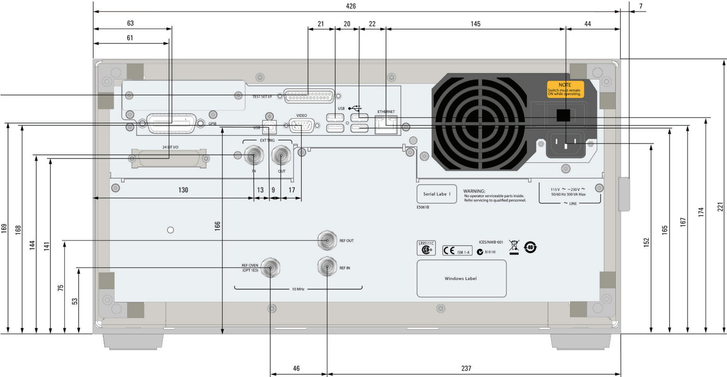
Figure 22. Dimensions (rear view, in millimeters)
