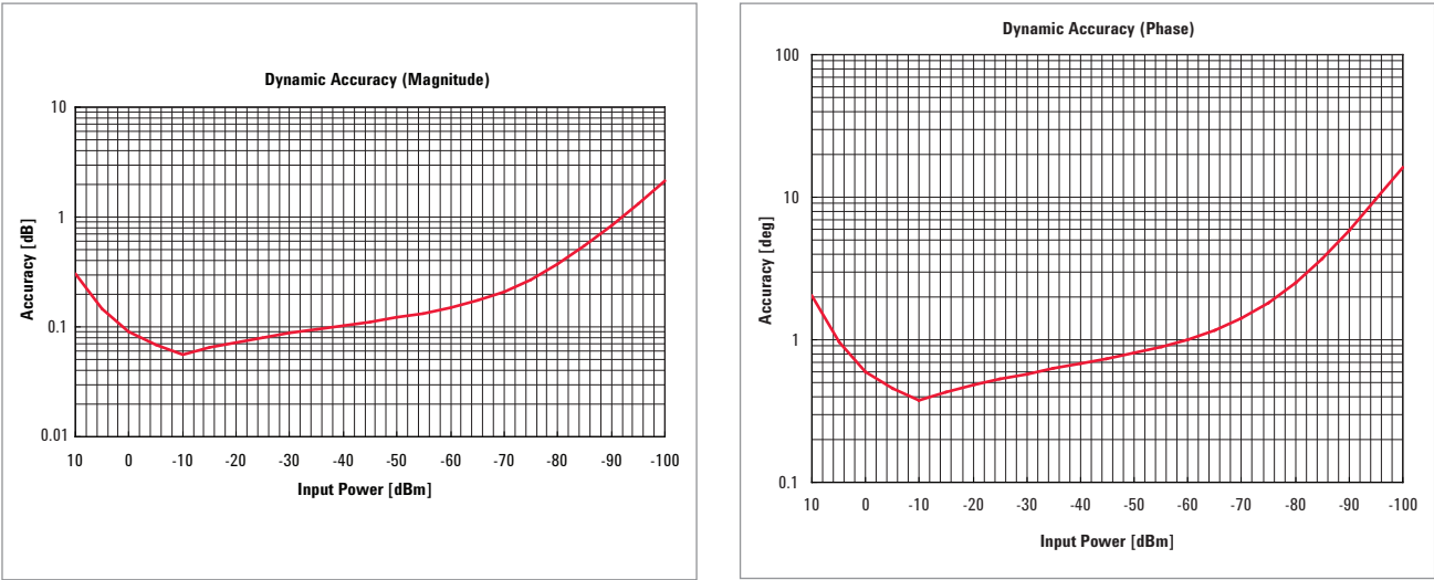
Figure 17. Dynamic Accuracy Option 3L3/3L4/3L5
