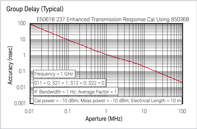
Figure 19. Group delay (typical)
