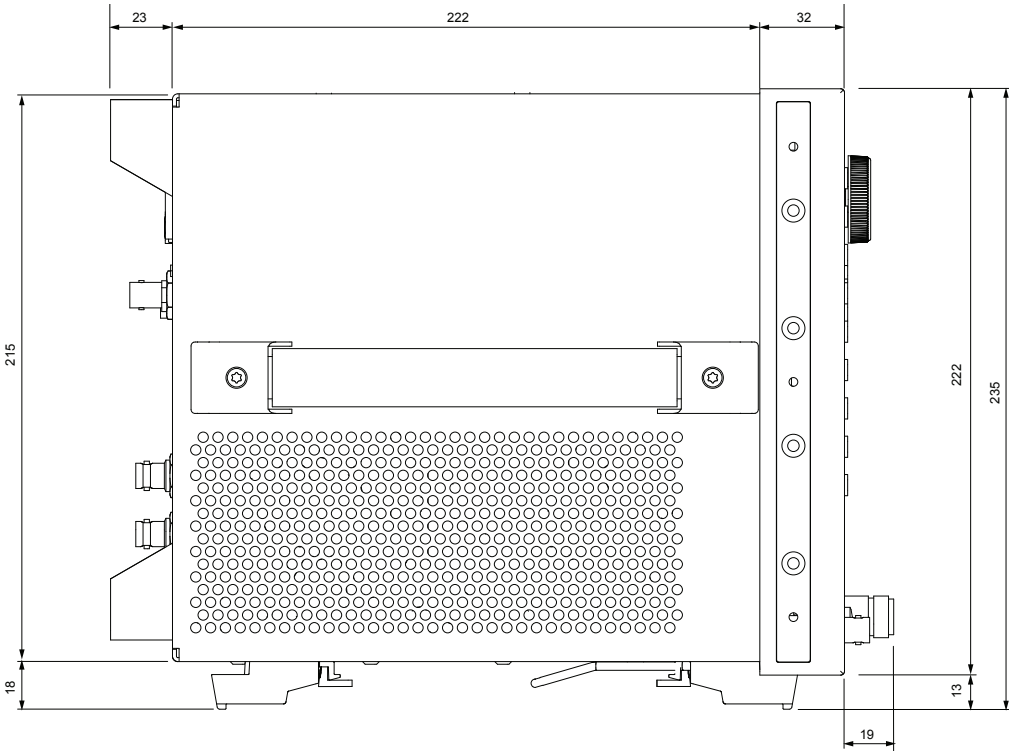
Figure 23. Dimensions (side view, in millimeters)
