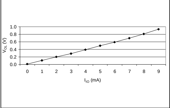
Figure 81. Typical V_{OL} at V_{DD}=5V ( \overline{RESET} )
