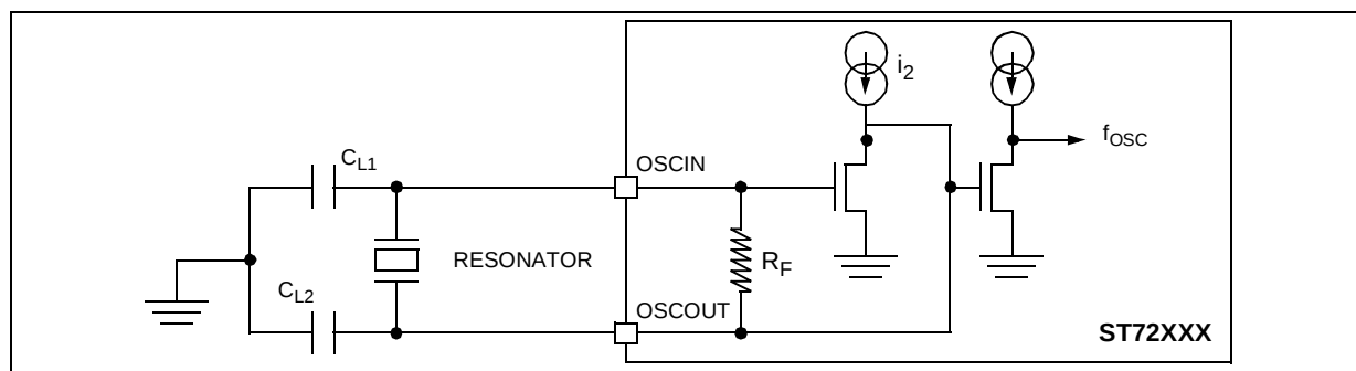
Figure 60. Typical Application with a Crystal Resonator
