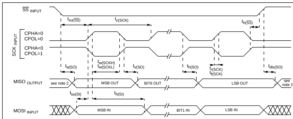
Figure 84. SPI Slave Timing Diagram with CPHA=0 3)
