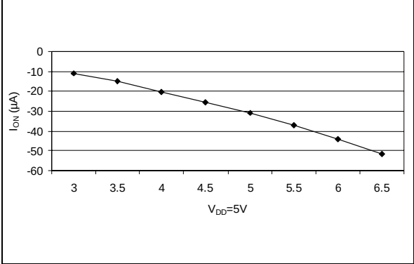
Figure 80. Typical I_{ON} vs. V_{DD} with V_{IN}=V_{SS}
