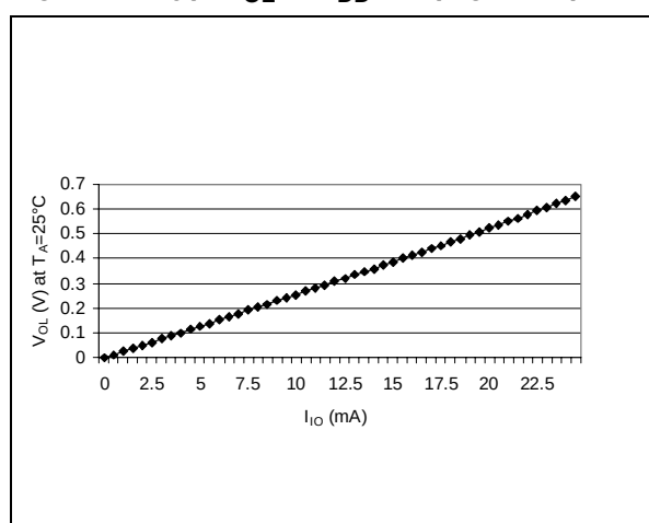
Figure 73. Typ. V_{OL} at V_{DD}=5V (high-sink)
