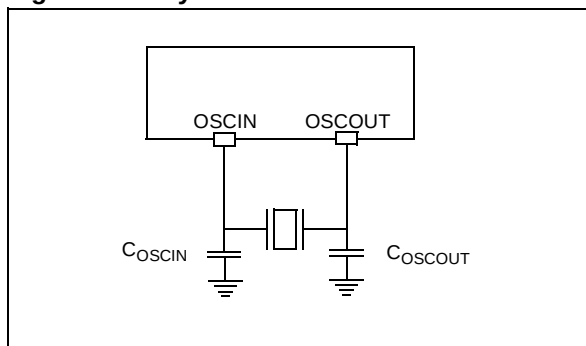
Figure 13. Crystal/Ceramic Resonator
