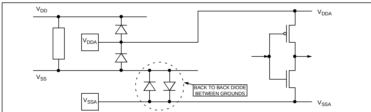
Figure 68. Multisupply Configuration
