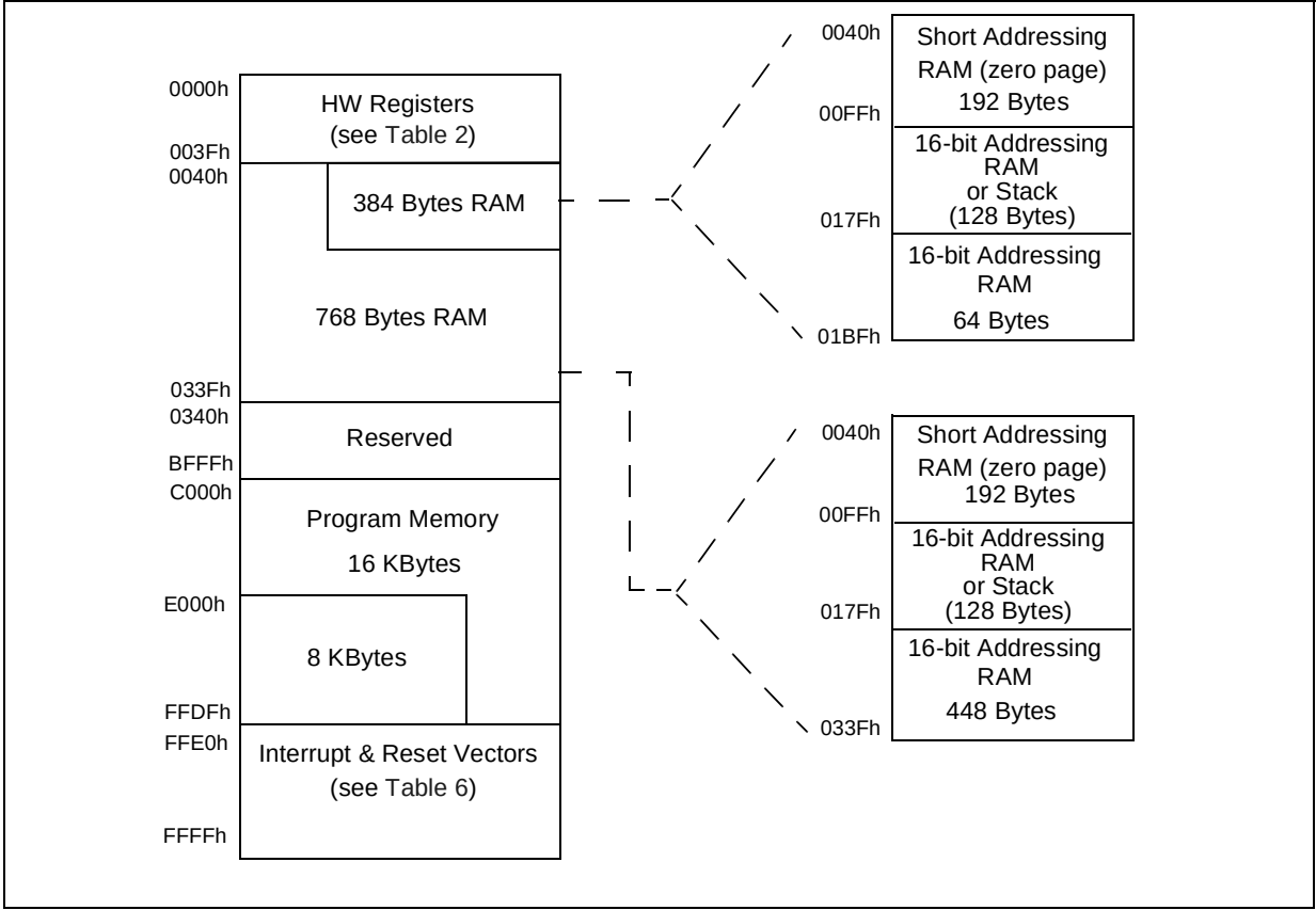
Figure 7. Memory Map
