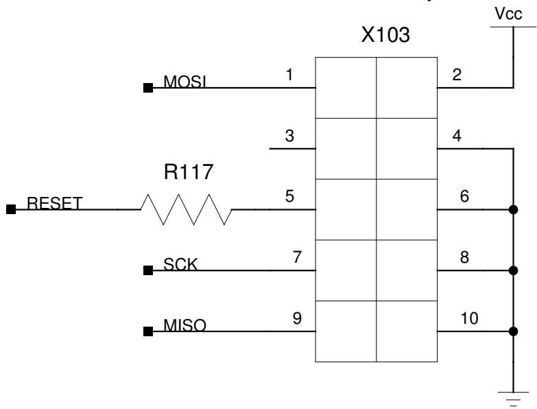
ISP socket --- standard STK200 layout
