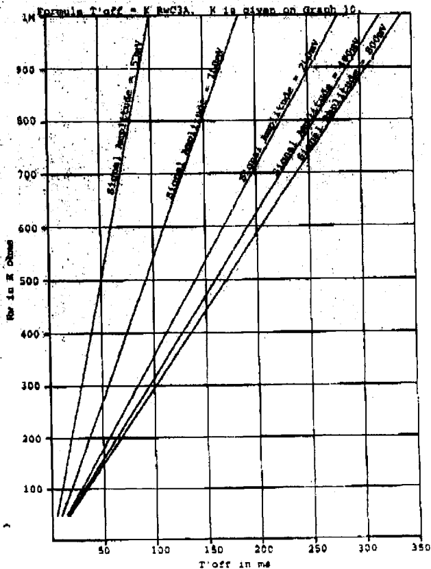
GRAPH 9 Graph showing T'off time for a given signal amplitude C3 = 0.1uF and Diode D1 between C3A & C3B.
