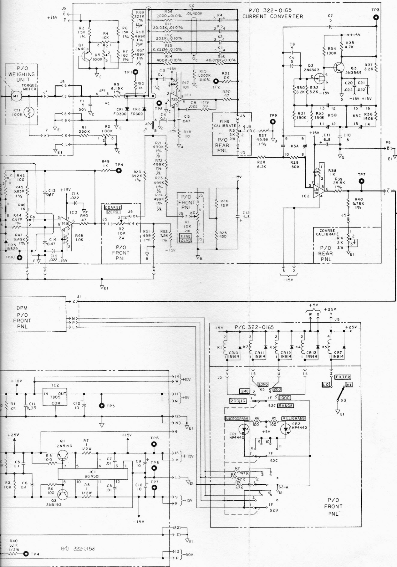
Fig. 6-1 - AM-2 Electrical Schematic (322-0171E)
