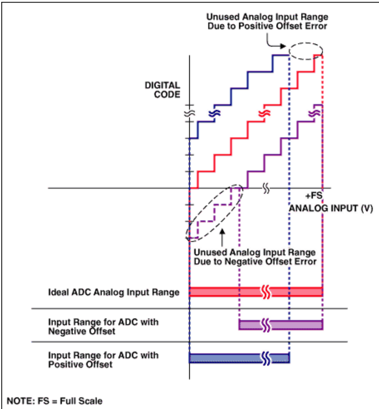
Figure 4. Unipolar offset error.
