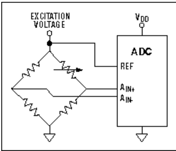
Figure 8. Ratiometric ADC conversion.
