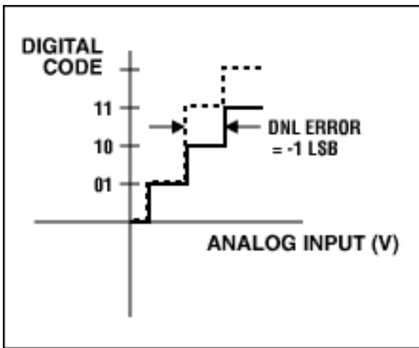
Figure 1c. DNL error: Code 10 is missing.
