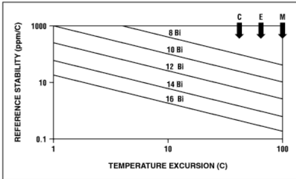
Figure 7. Voltage-reference-drift requirements relate to ADC resolution.
