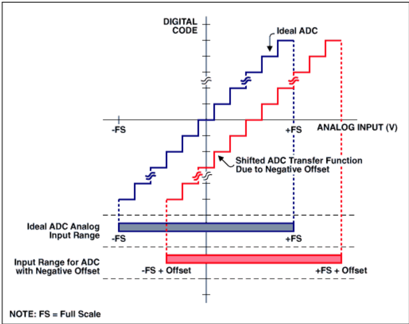
Figure 2. Bipolar offset error.
