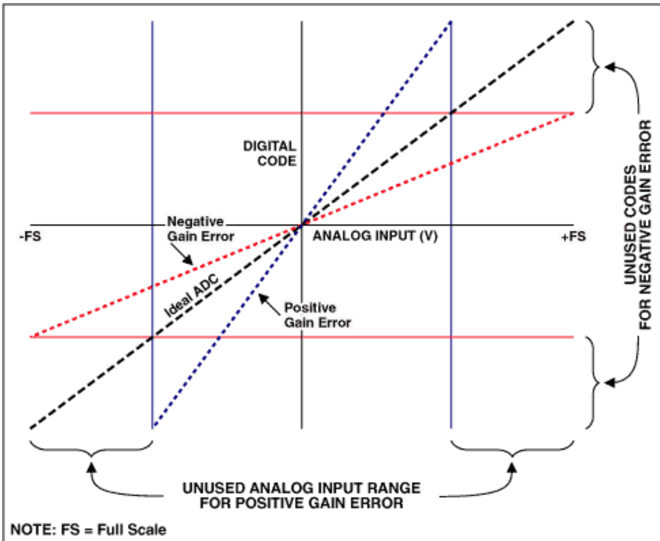
Figure 6. Gain error reduces dynamic range.
