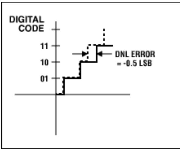
Figure 1b. DNL error: no missing codes.
