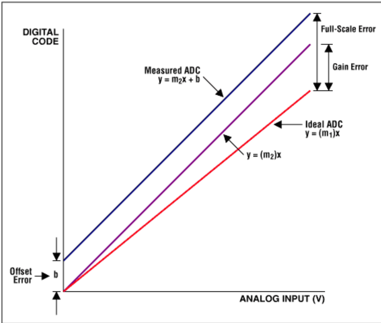
Figure 5. Offset, gain, and full-scale errors.
