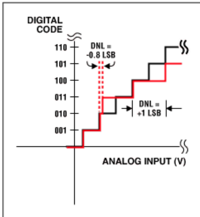
Figure 1a. DNL error: no missing codes.
