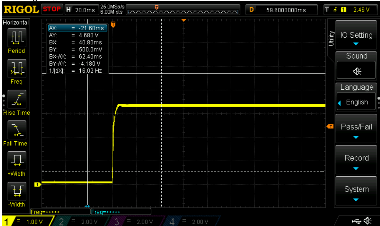
Switching ON, 3.3V with 1000mA load current
