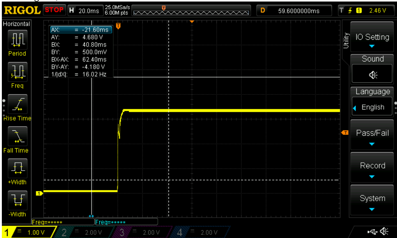
Switching ON, 3.3V with 100mA load current
